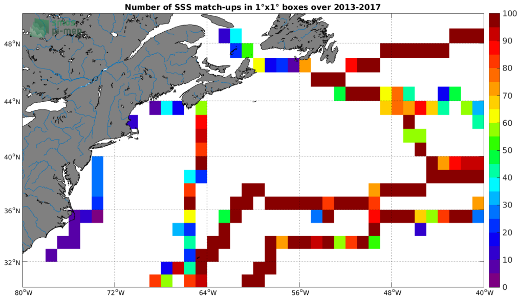
Figure 4: Number of SSS match-ups between TSG-GOSUD-Sailing-ship SSS and the SMOS-L3-CATDS-CPDC-V317-10DAYS-25KM SSS product for the Gulf Stream Pi-MEP region over 1°x1° boxes and for the full satellite product period.
