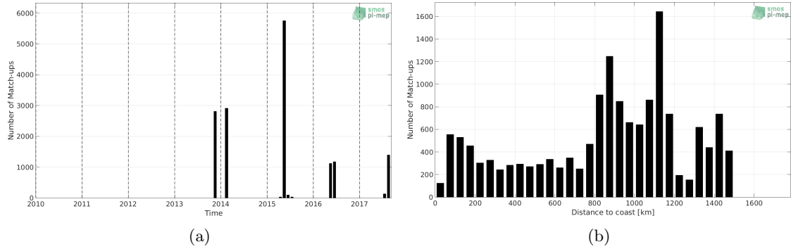
Figure 1: Number of match-ups between TSG-GOSUD-Sailing-ship and SMOS-L3-CATDS-CPDC-V317-10DAYS-25KM SSS as a function of time (a) and as function of the distance to coast (b) over the Gulf Stream Pi-MEP region and for the full satellite product period.
