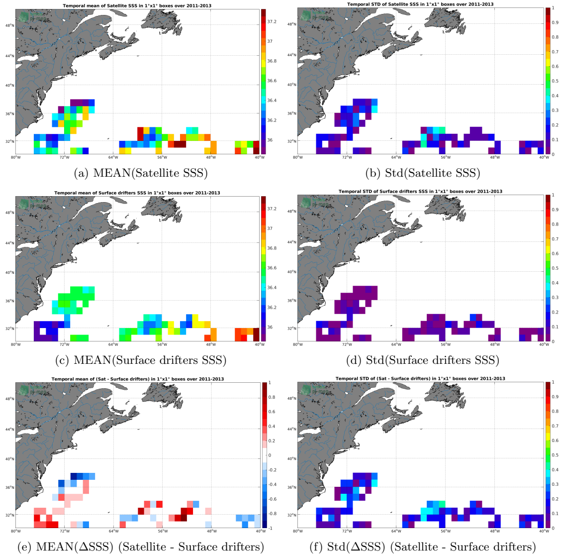
Figure 5: Temporal mean (left) and Std (right) of SSS from SMOS SSS L3 v317 - 10 Days - 25 km (CATDS-CPDC) (top), Surface drifters (middle), and of \Delta SSS (Satellite - Surface drifters). Only match-up pairs are used to generate these maps.
