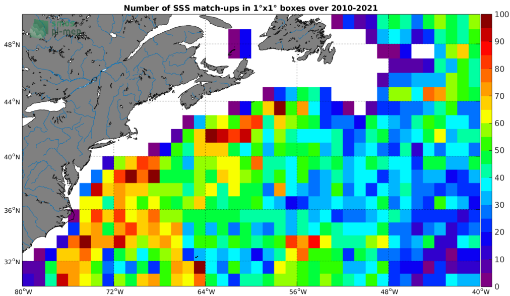
Figure 4: Number of SSS match-ups between Argo SSS and the SMOS SSS L3 v317 - 10 Days - 25 km (CATDS-CPDC) SSS product for the Gulf Stream Pi-MEP region over 1^\circ \times 1^\circ boxes and for the full satellite product period.
