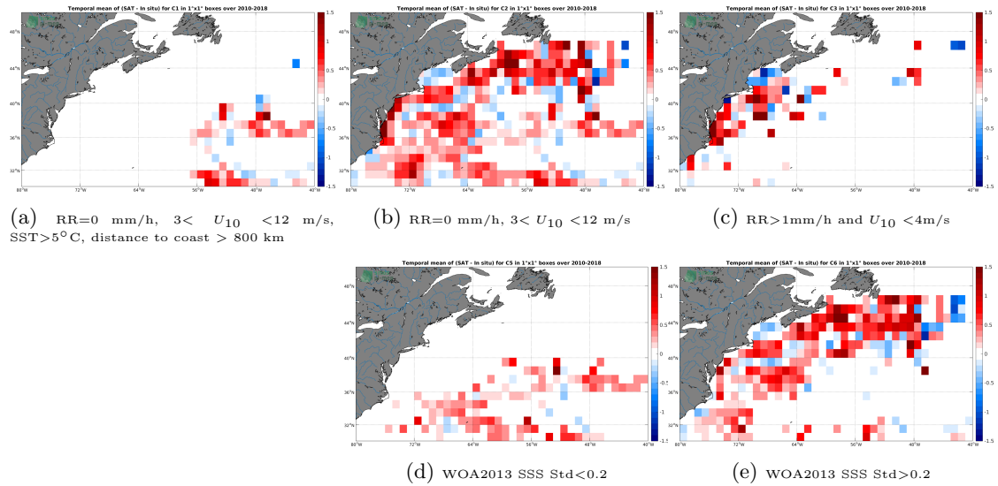
Figure 12: Temporal mean gridded over spatial boxes of size 1^\circ \times 1^\circ of \Delta SSS (SMOS-L3-CATDS-CPDC-V3-MONTHLY-25KM - TSG-SAMOS) for 5 different subdatasets corresponding to:RR=0 mm/h, 3 < U_{10} < 12 m/s, SST >5^\circ C, distance to coast > 800 km (a), RR=0 mm/h, 3 < U_{10} < 12 m/s (b), RR >1 mm/h and U_{10} < 4 m/s (c), WOA2013 SSS Std <0.2 (d), WOA2013 SSS Std >0.2 (e).
