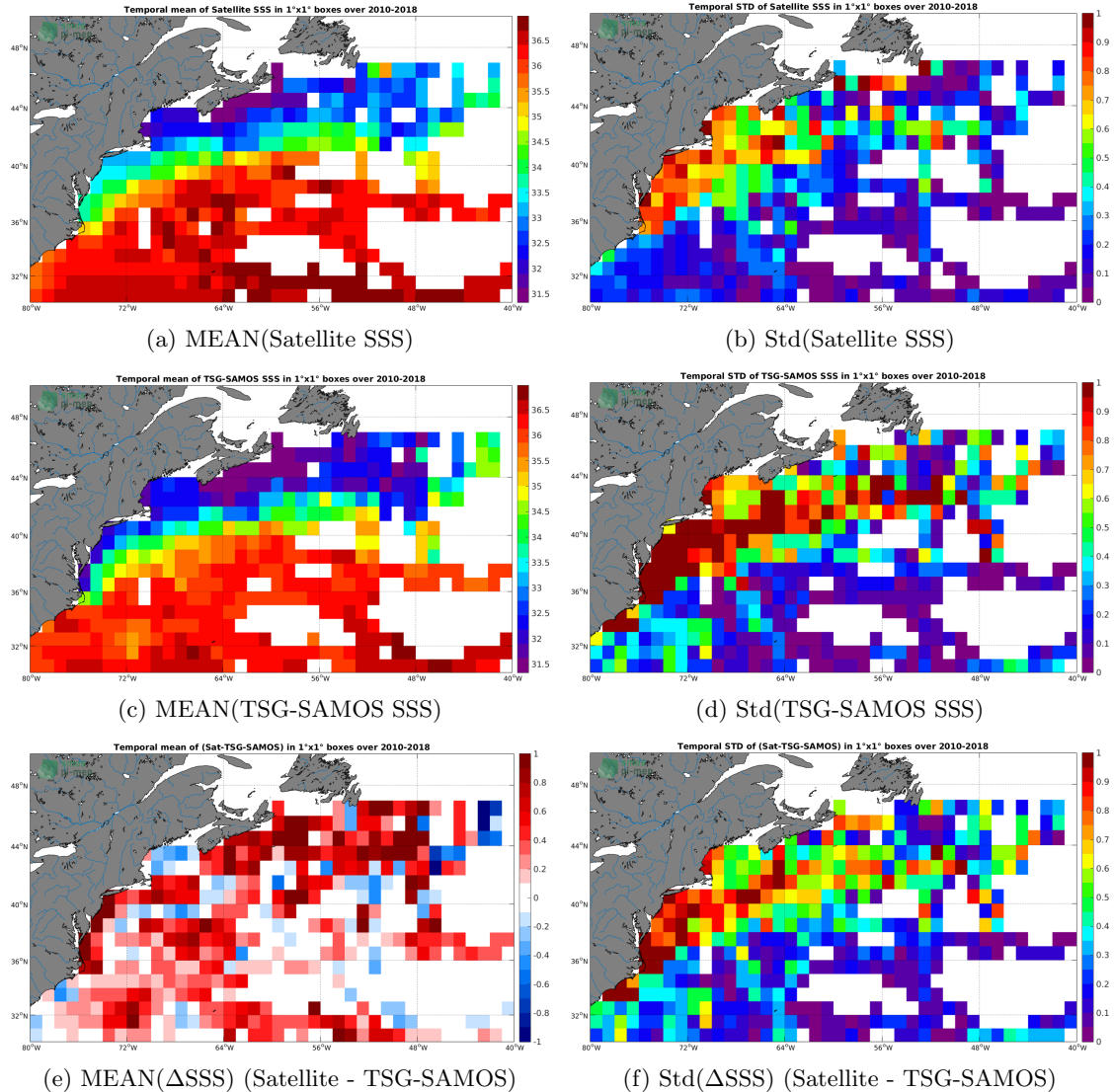
Figure 6: Temporal mean (left) and Std (right) of SSS from SMOS-L3-CATDS-CPDC-V3-MONTHLY-25KM (top), TSG-SAMOS (middle), and of \Delta SSS (Satellite - TSG-SAMOS). Only match-up pairs are used to generate these maps.
