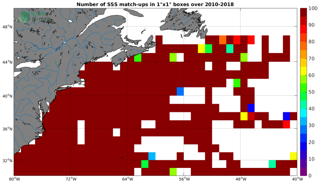
Figure 4: Number of SSS match-ups between TSG-SAMOS SSS and the SMOS-L3-CATDS-CPDC-V3-MONTHLY-25KM SSS product for the Gulf Stream Pi-MEP region over 1^\circ \times 1^\circ boxes and for the full satellite product period.
