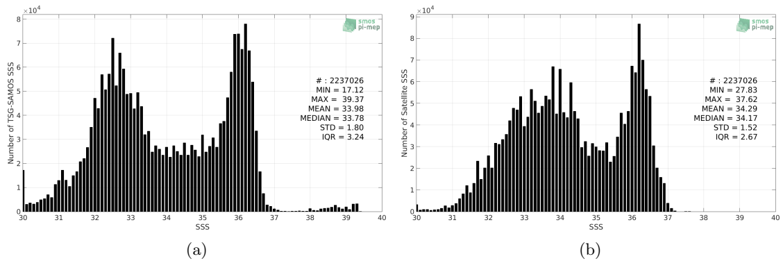
Figure 2: Histograms of SSS from TSG-SAMOS (a) and SMOS-L3-CATDS-CPDC-V3-MONTHLY-25KM (b) considering all match-up pairs per bins of 0.1 over the Gulf Stream Pi-MEP region and for the full satellite product period.
