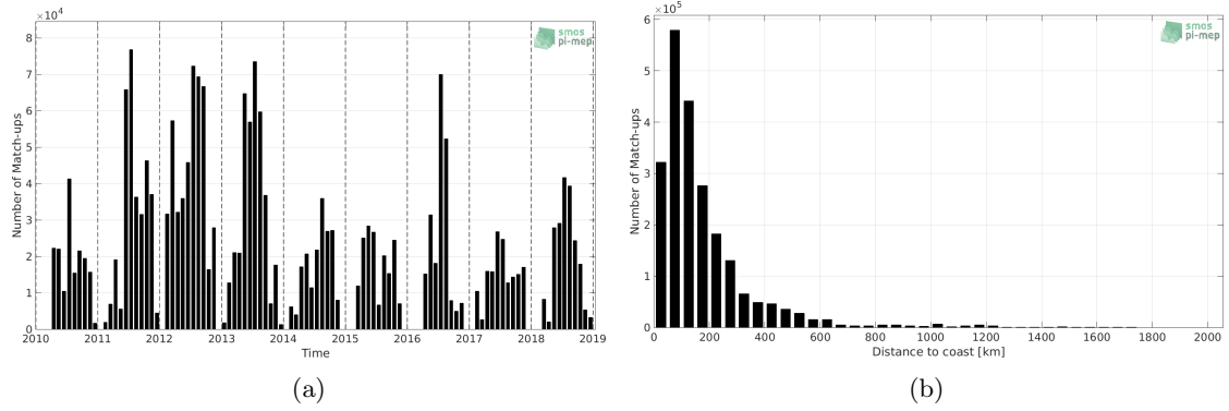
Figure 1: Number of match-ups between TSG-SAMOS and SMOS-L3-CATDS-CPDC-V3-MONTHLY-25KM SSS as a function of time (a) and as function of the distance to coast (b) over the Gulf Stream Pi-MEP region and for the full satellite product period.
