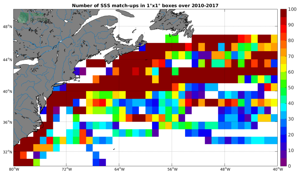
Figure 4: Number of SSS match-ups between TSG-LEGOS-DM SSS and the SMOS-L3-CATDS-CPDC-V3-MONTHLY-25KM SSS product for the Gulf Stream Pi-MEP region over 1^\circ \times 1^\circ boxes and for the full satellite product period.
