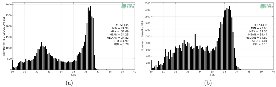
Figure 2: Histograms of SSS from TSG-LEGOS-DM (a) and SMOS-L3-CATDS-CPDC-V3-MONTHLY-25KM (b) considering all match-up pairs per bins of 0.1 over the Gulf Stream Pi-MEP region and for the full satellite product period.
