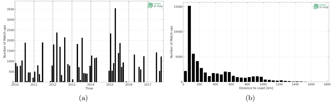
Figure 1: Number of match-ups between TSG-LEGOS-DM and SMOS-L3-CATDS-CPDC-V3-MONTHLY-25KM SSS as a function of time (a) and as function of the distance to coast (b) over the Gulf Stream Pi-MEP region and for the full satellite product period.
