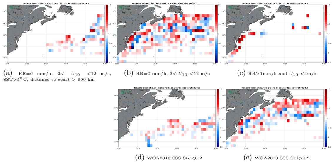
Figure 12: Temporal mean gridded over spatial boxes of size 1^\circ \times 1^\circ of \Delta SSS (SMOS-L3-CATDS-CPDC-V3-MONTHLY-25KM - TSG-LEGOS-DM) for 5 different subdatasets corresponding to:RR=0 mm/h, 3 < U_{10} < 12 m/s, SST >5^\circ C, distance to coast > 800 km (a), RR=0 mm/h, 3 < U_{10} < 12 m/s (b), RR >1 mm/h and U_{10} < 4 m/s (c), WOA2013 SSS Std <0.2 (d), WOA2013 SSS Std >0.2 (e).
