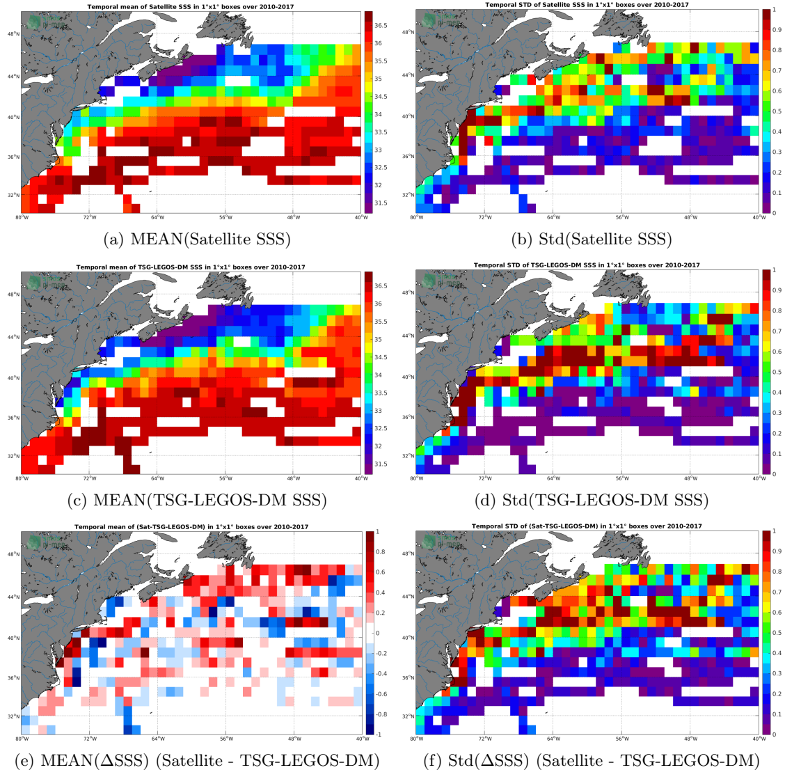
Figure 6: Temporal mean (left) and Std (right) of SSS from SMOS-L3-CATDS-CPDC-V3-MONTHLY-25KM (top), TSG-LEGOS-DM (middle), and of \Delta SSS (Satellite - TSG-LEGOS-DM). Only match-up pairs are used to generate these maps.
