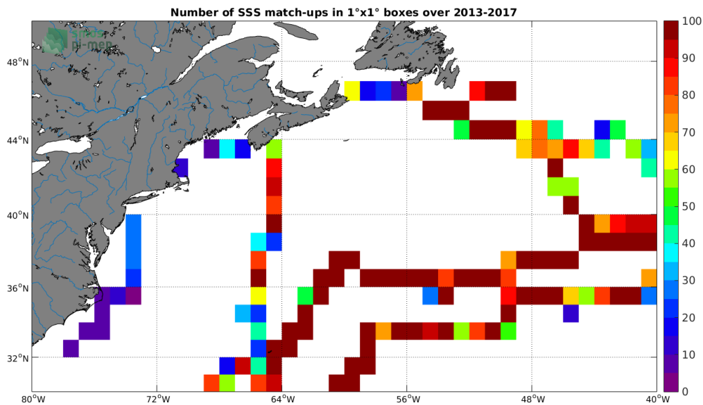
Figure 4: Number of SSS match-ups between TSG-GOSUD-Sailing-ship SSS and the SMOS-L3-CATDS-CPDC-V3-MONTHLY-25KM SSS product for the Gulf Stream Pi-MEP region over 1^\circ \times 1^\circ boxes and for the full satellite product period.
