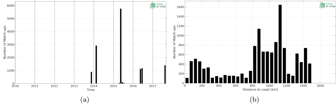
Figure 1: Number of match-ups between TSG-GOSUD-Sailing-ship and SMOS-L3-CATDS-CPDC-V3-MONTHLY-25KM SSS as a function of time (a) and as function of the distance to coast (b) over the Gulf Stream Pi-MEP region and for the full satellite product period.
