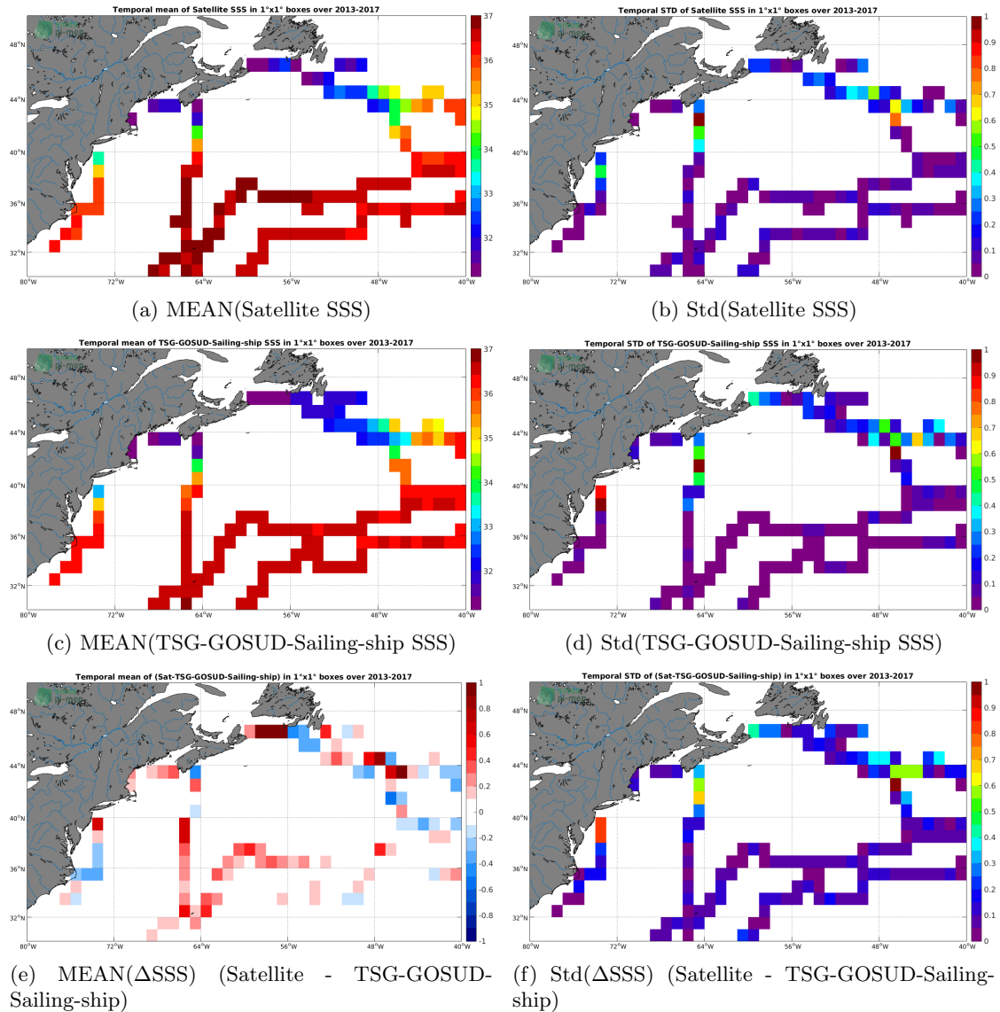
Figure 6: Temporal mean (left) and Std (right) of SSS from SMOS-L3-CATDS-CPDC-V3-MONTHLY-25KM (top), TSG-GOSUD-Sailing-ship (middle), and of \Delta SSS (Satellite - TSG-GOSUD-Sailing-ship). Only match-up pairs are used to generate these maps.
