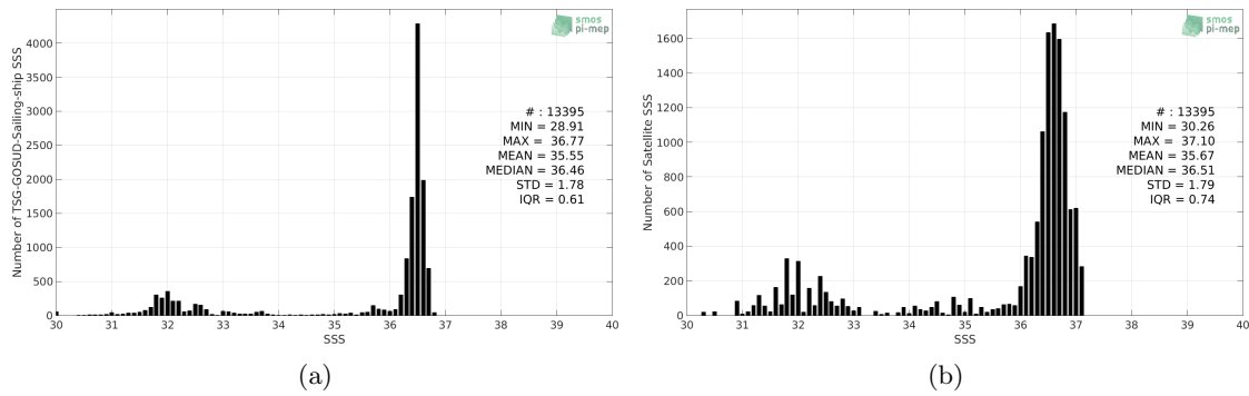
Figure 2: Histograms of SSS from TSG-GOSUD-Sailing-ship (a) and SMOS-L3-CATDS-CPDC-V3-MONTHLY-25KM (b) considering all match-up pairs per bins of 0.1 over the Gulf Stream Pi-MEP region and for the full satellite product period.
