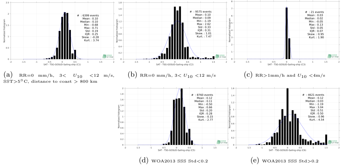
Figure 13: Normalized histogram of \Delta\text{SSS} (SMOS-L3-CATDS-CPDC-V3-MONTHLY-25KM - TSG-GOSUD-Sailing-ship) for 5 different subdatasets corresponding to: RR=0 mm/h, 3 < U_{10} < 12 m/s, SST > 5^\circ\text{C} , distance to coast > 800 km (a), RR=0 mm/h, 3 < U_{10} < 12 m/s (b), RR > 1\text{mm/h} and U_{10} < 4\text{m/s} (c), WOA2013 SSS Std < 0.2 (d), WOA2013 SSS Std > 0.2 (e).
