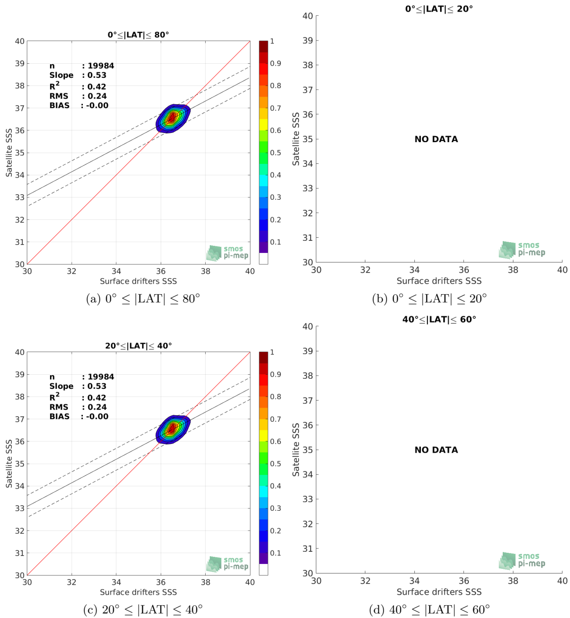
Figure 8: Contour maps of the concentration of SMOS-L3-CATDS-CPDC-V3-MONTHLY-25KM SSS (y-axis) versus Surface drifters SSS (x-axis) at match-up pairs for different latitude bands. For each plot, the red line shows x=y . The black thin and dashed lines indicate a linear fit through the data cloud and the \pm 95\% confidence levels, respectively. The number match-up pairs n , the slope and R^2 coefficient of the linear fit, the root mean square (RMS) and the mean bias between satellite and in situ data are indicated for each latitude band in each plots.
