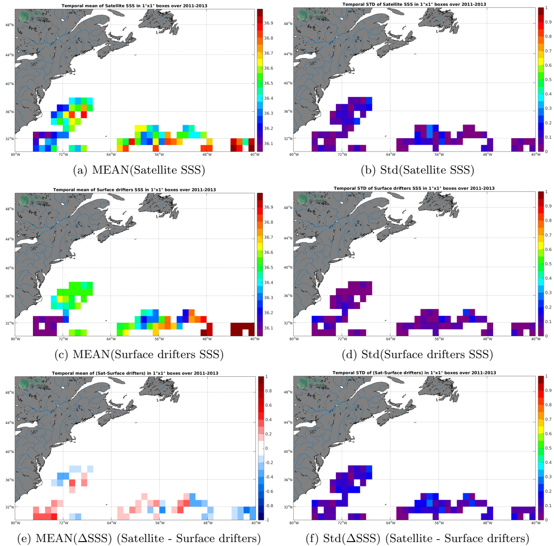
Figure 5: Temporal mean (left) and Std (right) of SSS from SMOS-L3-CATDS-CPDC-V3-MONTHLY-25KM (top), Surface drifters (middle), and of \Delta SSS (Satellite - Surface drifters). Only match-up pairs are used to generate these maps.
