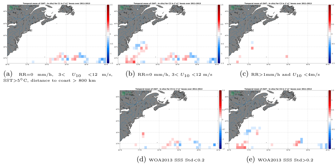
Figure 11: Temporal mean gridded over spatial boxes of size 1^\circ \times 1^\circ of \Delta SSS (SMOS-L3-CATDS-CPDC-V3-MONTHLY-25KM - Surface drifters) for 5 different subdatasets corresponding to: RR=0 mm/h, 3 < U_{10} < 12 m/s, SST > 5^\circ C , distance to coast > 800 km (a), RR=0 mm/h, 3 < U_{10} < 12 m/s (b), RR > 1 mm/h and U_{10} < 4 m/s (c), WOA2013 SSS Std < 0.2 (d), WOA2013 SSS Std > 0.2 (e).
