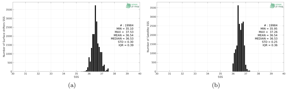
Figure 2: Histograms of SSS from Surface drifters (a) and SMOS-L3-CATDS-CPDC-V3-MONTHLY-25KM (b) considering all match-up pairs per bins of 0.1 over the Gulf Stream Pi-MEP region and for the full satellite product period.
