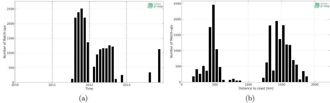
Figure 1: Number of match-ups between Surface drifters and SMOS-L3-CATDS-CPDC-V3-MONTHLY-25KM SSS as a function of time (a) and as function of the distance to coast (b) over the Gulf Stream Pi-MEP region and for the full satellite product period.
