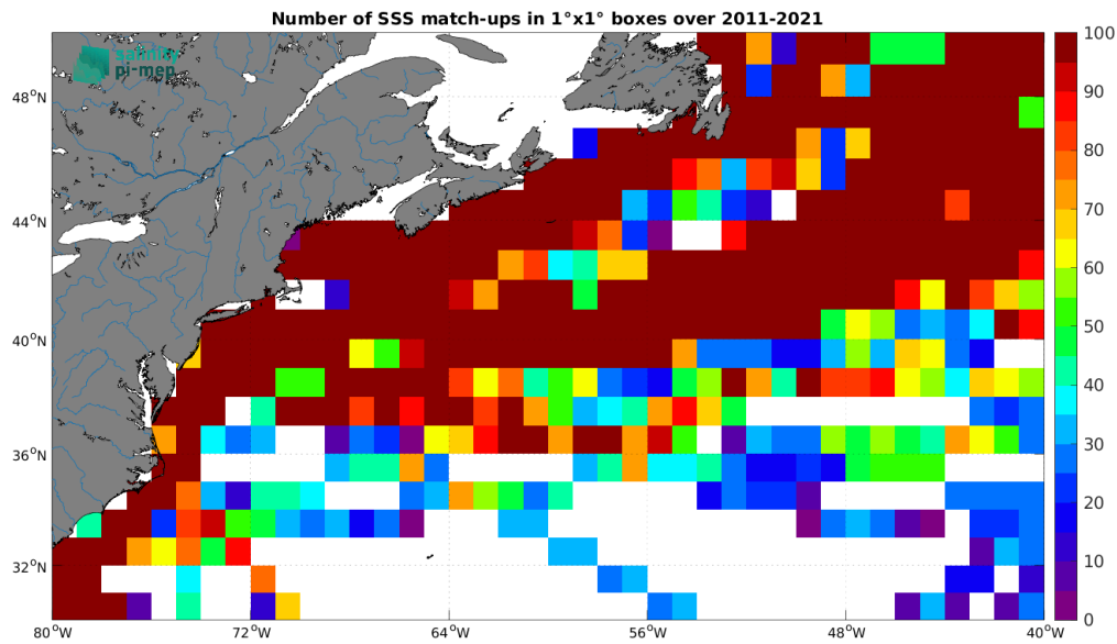
Figure 5: Number of SSS match-ups between TSG (LEGOS-DM) SSS and the SMOS SSS L3 v2 - 9-Days (BEC) SSS product for the Gulf Stream Pi-MEP region over 1^\circ \times 1^\circ boxes and for the full satellite product period.
