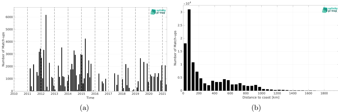
Figure 2: Number of match-ups between TSG (LEGOS-DM) and SMOS SSS L3 v2 - 9-Days (BEC) SSS as a function of time (a) and as function of the distance to coast (b) over the Gulf Stream Pi-MEP region and for the full satellite product period.
