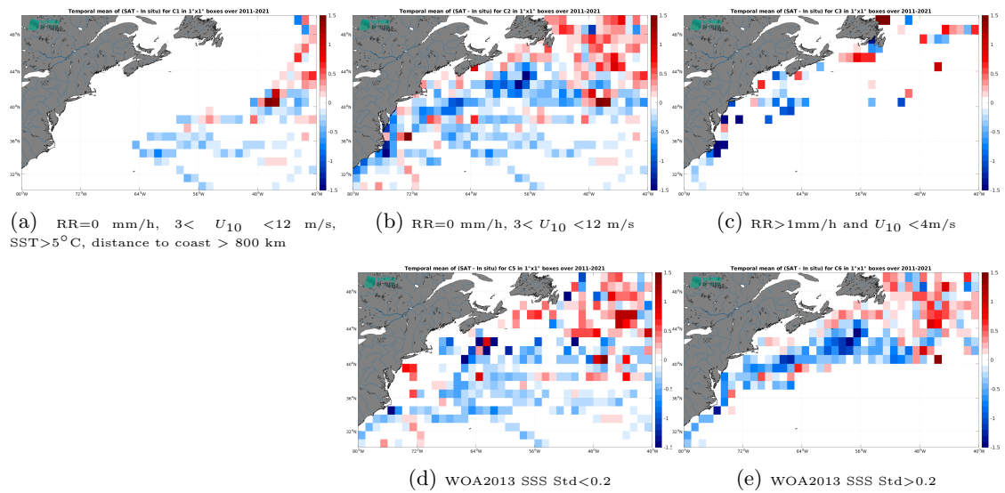
Figure 14: Temporal mean gridded over spatial boxes of size 1^\circ \times 1^\circ of \Delta SSS (SMOS SSS L3 v2 - 9-Days (BEC) - TSG (LEGOS-DM)) for 5 different subdatasets corresponding to: RR=0 mm/h, 3 < U_{10} < 12 m/s, SST > 5°C, distance to coast > 800 km (a), RR=0 mm/h, 3 < U_{10} < 12 m/s (b), RR > 1mm/h and U_{10} < 4 m/s (c), WOA2013 SSS Std < 0.2 (d), WOA2013 SSS Std > 0.2 (e).
