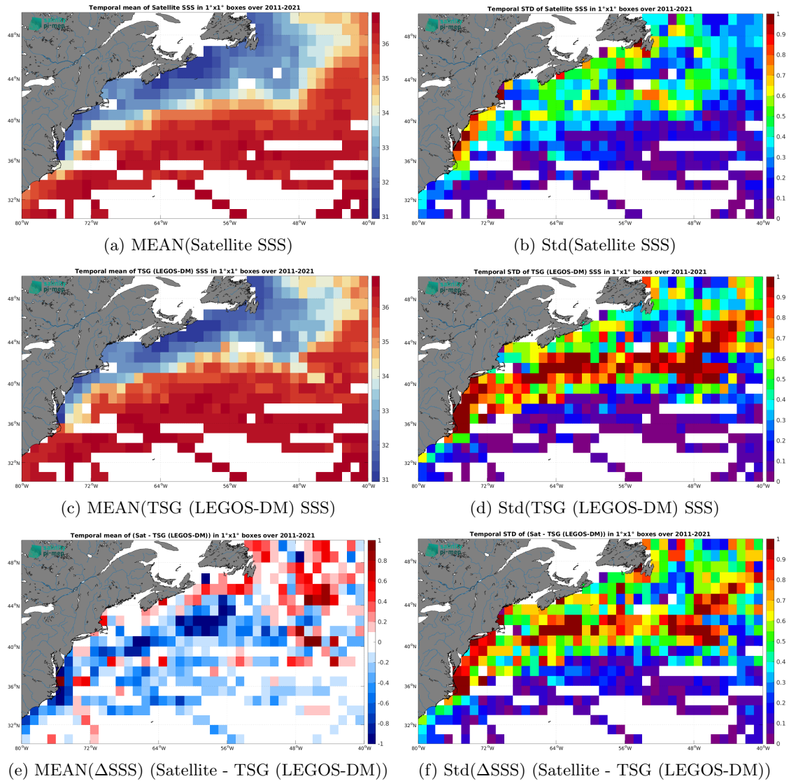
Figure 7: Temporal mean (left) and Std (right) of SSS from SMOS SSS L3 v2 - 9-Days (BEC) (top), TSG (LEGOS-DM) (middle), and of \Delta SSS (Satellite - TSG (LEGOS-DM)). Only match-up pairs are used to generate these maps.
