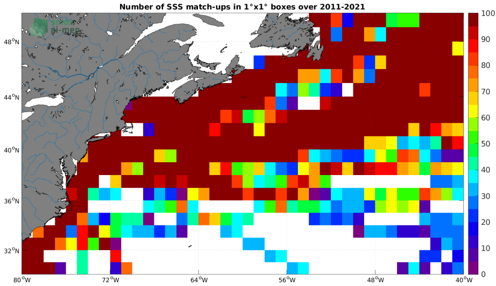
Figure 4: Number of SSS match-ups between TSG (LEGOS-DM) SSS and the SMOS SSS L3 v2 - 9-Days (BEC) SSS product for the Gulf Stream Pi-MEP region over 1^{\circ} \times 1^{\circ} boxes and for the full satellite product period.
