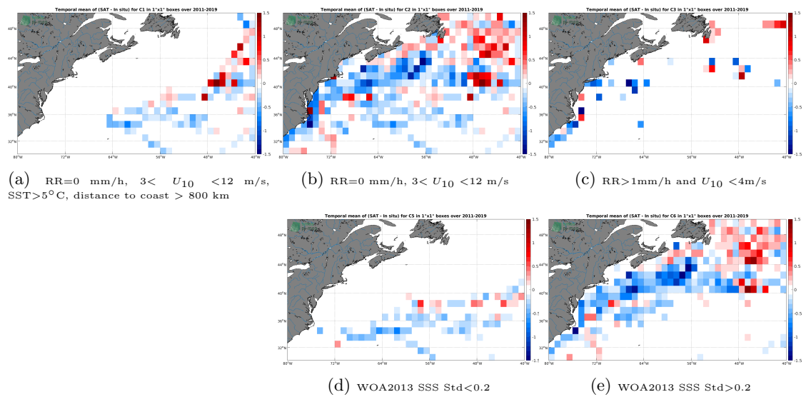
Figure 12: Temporal mean gridded over spatial boxes of size 1°x1° of \Delta SSS (SMOS SSS L3 v2 - 9-Days (BEC) - TSG (LEGOS-DM)) for 5 different subdatasets corresponding to:RR=0 mm/h, 3 < U_{10} < 12 m/s, SST>5°C, distance to coast > 800 km (a), RR=0 mm/h, 3 < U_{10} < 12 m/s (b), RR>1mm/h and U_{10} < 4 m/s (c), WOA2013 SSS Std<0.2 (d), WOA2013 SSS Std>0.2 (e).
