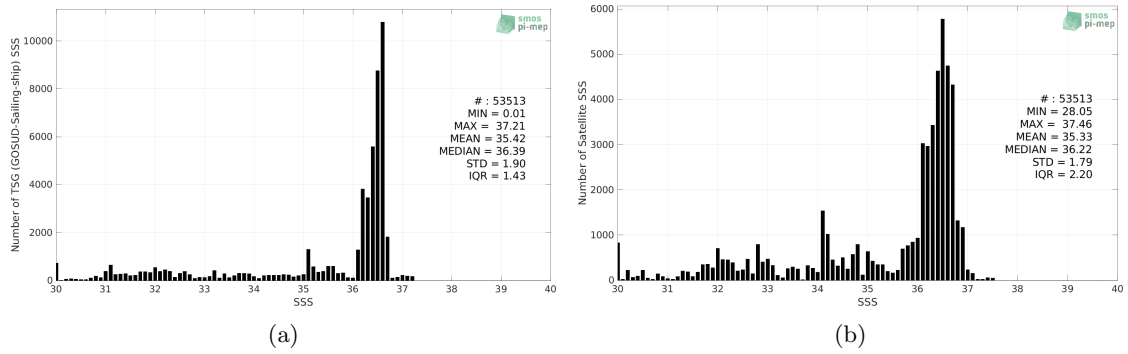
Figure 2: Histograms of SSS from TSG (GOSUD-Sailing-ship) (a) and SMOS SSS L3 v2 - 9-Days (BEC) (b) considering all match-up pairs per bins of 0.1 over the Gulf Stream Pi-MEP region and for the full satellite product period.
