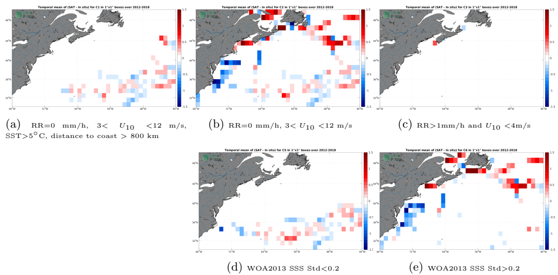
Figure 12: Temporal mean gridded over spatial boxes of size 1^\circ \times 1^\circ of \Delta SSS (SMOS SSS L3 v2 - 9-Days (BEC) - TSG (GOSUD-Sailing-ship)) for 5 different subdatasets corresponding to:RR=0 mm/h, 3 < U_{10} < 12 m/s, SST > 5°C, distance to coast > 800 km (a), RR=0 mm/h, 3 < U_{10} < 12 m/s (b), RR > 1mm/h and U_{10} < 4 m/s (c), WOA2013 SSS Std < 0.2 (d), WOA2013 SSS Std > 0.2 (e).
