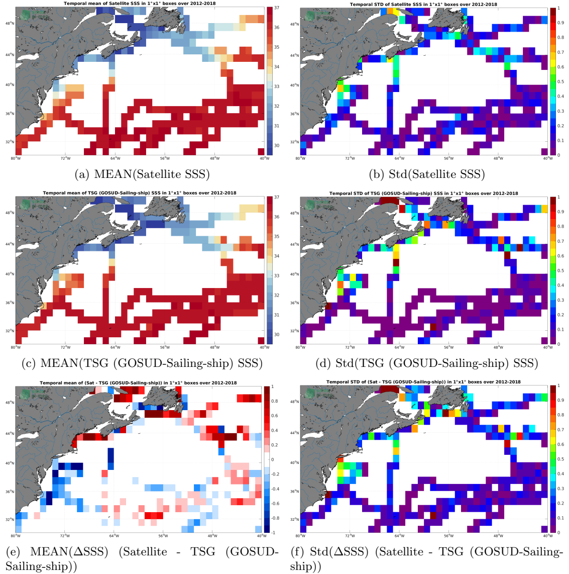
Figure 6: Temporal mean (left) and Std (right) of SSS from SMOS SSS L3 v2 - 9-Days (BEC) (top), TSG (GOSUD-Sailing-ship) (middle), and of \Delta SSS (Satellite - TSG (GOSUD-Sailing-ship)). Only match-up pairs are used to generate these maps.
