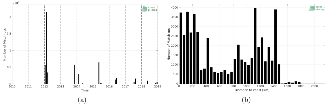
Figure 1: Number of match-ups between TSG (GOSUD-Sailing-ship) and SMOS SSS L3 v2 - 9-Days (BEC) SSS as a function of time (a) and as function of the distance to coast (b) over the Gulf Stream Pi-MEP region and for the full satellite product period.
