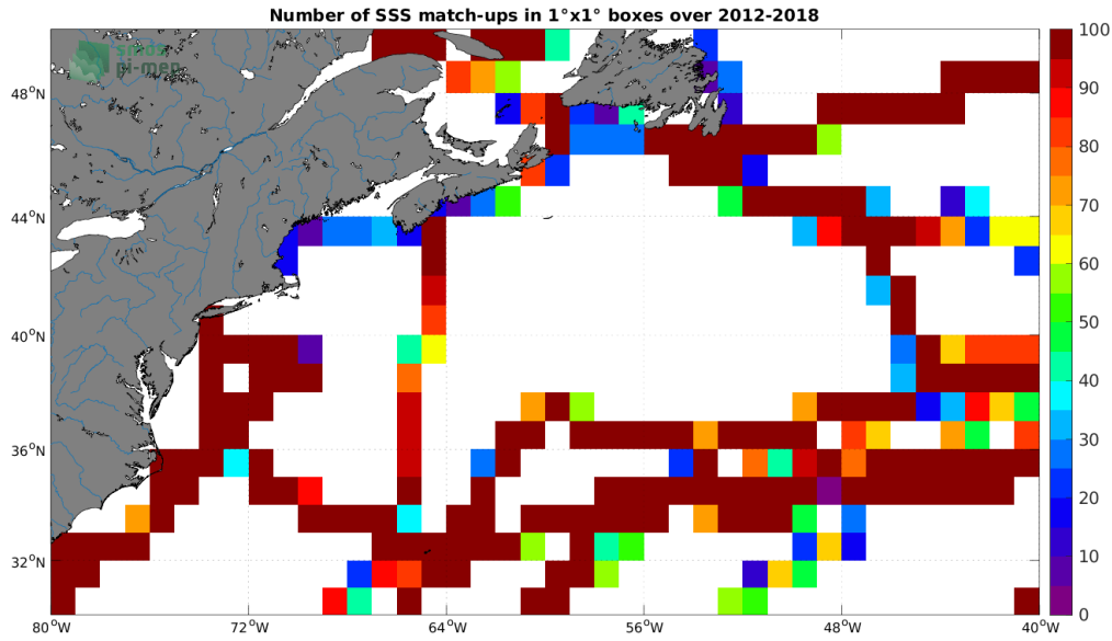
Figure 4: Number of SSS match-ups between TSG (GOSUD-Sailing-ship) SSS and the SMOS SSS L3 v2 - 9-Days (BEC) SSS product for the Gulf Stream Pi-MEP region over 1^\circ \times 1^\circ boxes and for the full satellite product period.
