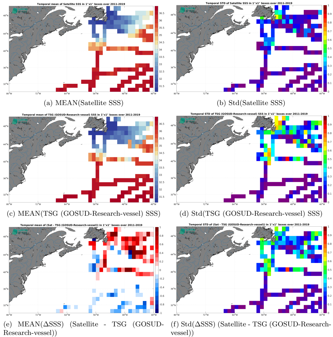
Figure 7: Temporal mean (left) and Std (right) of SSS from SMOS SSS L3 v2 - 9-Days (BEC) (top), TSG (GOSUD-Research-vessel) (middle), and of \Delta SSS (Satellite - TSG (GOSUD-Research-vessel)). Only match-up pairs are used to generate these maps.
