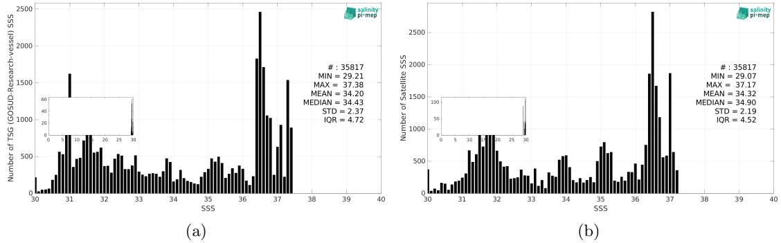
Figure 3: Histograms of SSS from TSG (GOSUD-Research-vessel) (a) and SMOS SSS L3 v2 - 9-Days (BEC) (b) considering all match-up pairs per bins of 0.1 over the Gulf Stream Pi-MEP region and for the full satellite product period.
