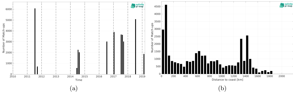
Figure 2: Number of match-ups between TSG (GOSUD-Research-vessel) and SMOS SSS L3 v2 - 9-Days (BEC) SSS as a function of time (a) and as function of the distance to coast (b) over the Gulf Stream Pi-MEP region and for the full satellite product period.
