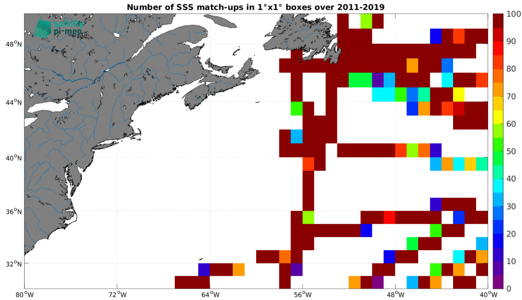
Figure 5: Number of SSS match-ups between TSG (GOSUD-Research-vessel) SSS and the SMOS SSS L3 v2 - 9-Days (BEC) SSS product for the Gulf Stream Pi-MEP region over 1^\circ \times 1^\circ boxes and for the full satellite product period.
