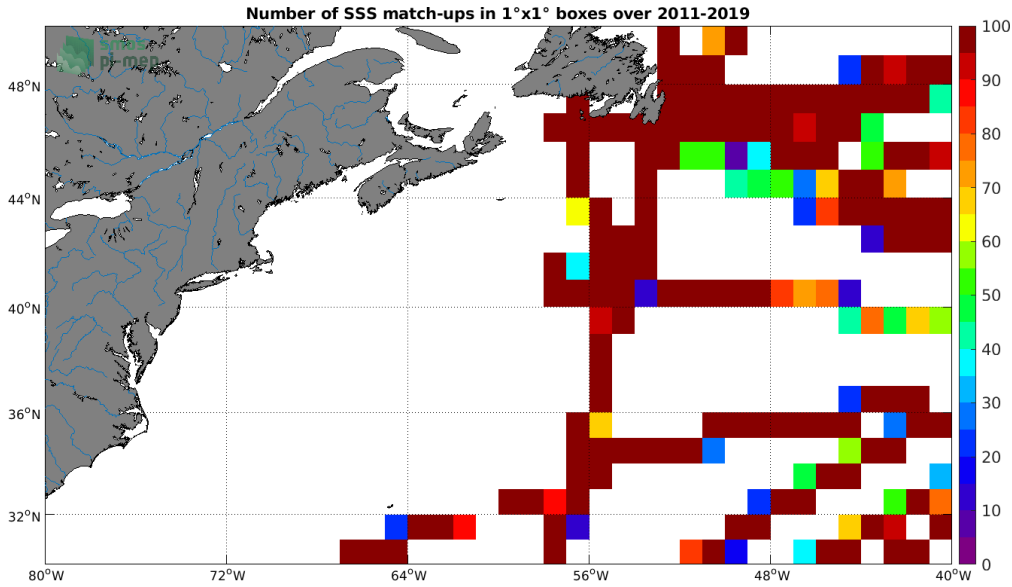
Figure 4: Number of SSS match-ups between TSG (GOSUD-Research-vessel) SSS and the SMOS SSS L3 v2 - 9-Days (BEC) SSS product for the Gulf Stream Pi-MEP region over 1^{\circ} \times 1^{\circ} boxes and for the full satellite product period.
