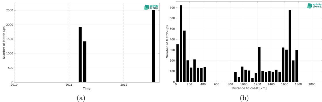
Figure 2: Number of match-ups between TSG (CSIC-UTM) and SMOS SSS L3 v2 - 9-Days (BEC) SSS as a function of time (a) and as function of the distance to coast (b) over the Gulf Stream Pi-MEP region and for the full satellite product period.
