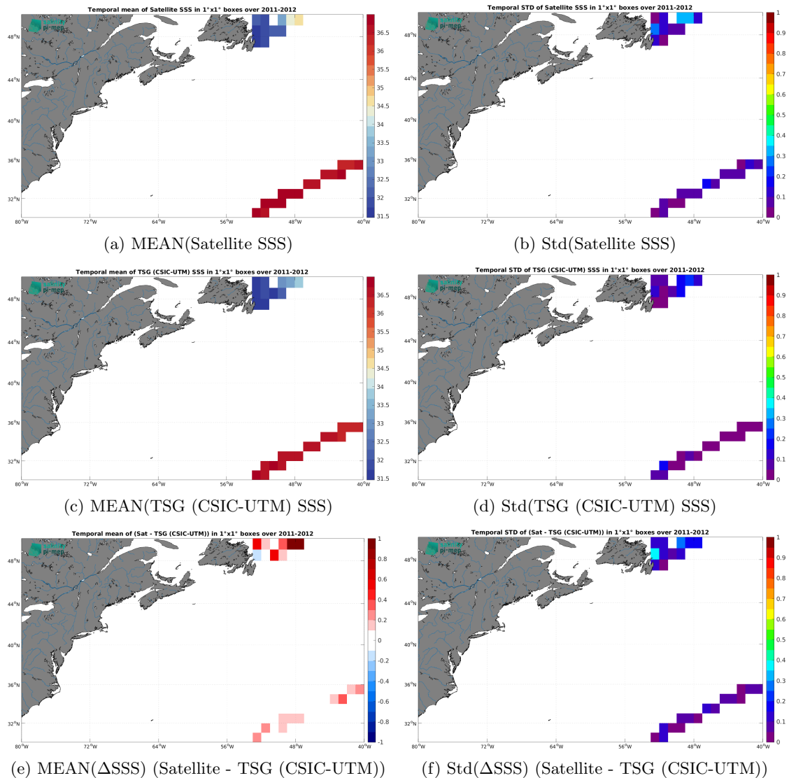
Figure 7: Temporal mean (left) and Std (right) of SSS from SMOS SSS L3 v2 - 9-Days (BEC) (top), TSG (CSIC-UTM) (middle), and of \Delta SSS (Satellite - TSG (CSIC-UTM)). Only match-up pairs are used to generate these maps.
