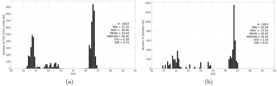
Figure 3: Histograms of SSS from TSG (CSIC-UTM) (a) and SMOS SSS L3 v2 - 9-Days (BEC) (b) considering all match-up pairs per bins of 0.1 over the Gulf Stream Pi-MEP region and for the full satellite product period.
