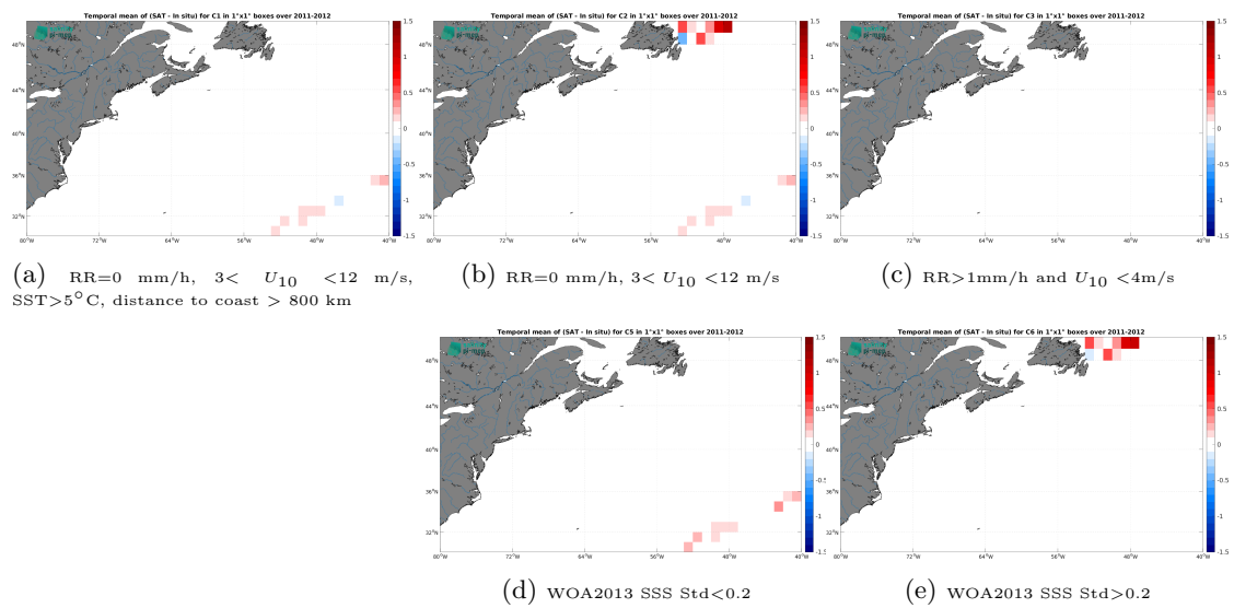
Figure 14: Temporal mean gridded over spatial boxes of size 1^\circ \times 1^\circ of \Delta SSS (SMOS SSS L3 v2 - 9-Days (BEC) - TSG (CSIC-UTM)) for 5 different subdatasets corresponding to: RR=0 mm/h, 3 < U_{10} < 12 m/s, SST > 5°C, distance to coast > 800 km (a), RR=0 mm/h, 3 < U_{10} < 12 m/s (b), RR > 1mm/h and U_{10} < 4 m/s (c), WOA2013 SSS Std < 0.2 (d), WOA2013 SSS Std > 0.2 (e).
