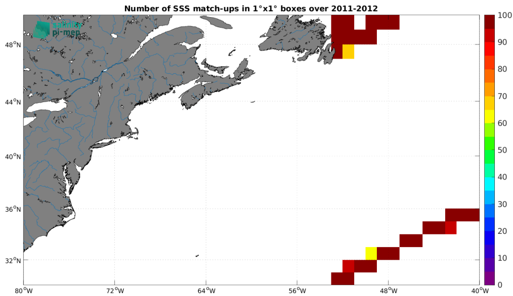
Figure 5: Number of SSS match-ups between TSG (CSIC-UTM) SSS and the SMOS SSS L3 v2 - 9-Days (BEC) SSS product for the Gulf Stream Pi-MEP region over 1^{\circ} \times 1^{\circ} boxes and for the full satellite product period.
