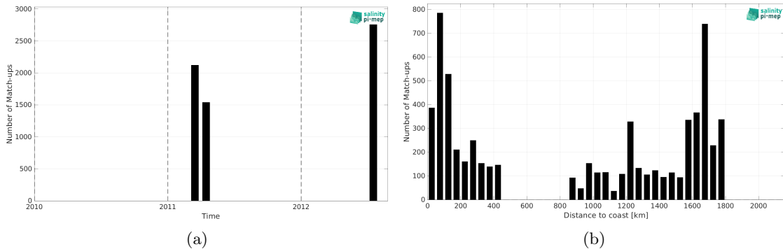
Figure 1: Number of match-ups between TSG (CSIC-UTM) and SMOS SSS L3 v2 - 9-Days (BEC) SSS as a function of time (a) and as function of the distance to coast (b) over the Gulf Stream Pi-MEP region and for the full satellite product period.
