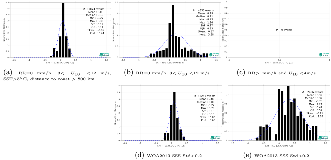
Figure 13: Normalized histogram of \Delta SSS (SMOS SSS L3 v2 - 9-Days (BEC) - TSG (CSIC-UTM)) for 5 different subdatasets corresponding to: RR=0 mm/h, 3 < U_{10} < 12 m/s, SST > 5°C, distance to coast > 800 km (a), RR=0 mm/h, 3 < U_{10} < 12 m/s (b), RR > 1mm/h and U_{10} < 4 m/s (c), WOA2013 SSS Std < 0.2 (d), WOA2013 SSS Std > 0.2 (e).
