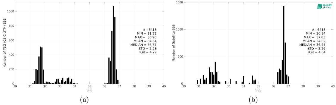
Figure 2: Histograms of SSS from TSG (CSIC-UTM) (a) and SMOS SSS L3 v2 - 9-Days (BEC) (b) considering all match-up pairs per bins of 0.1 over the Gulf Stream Pi-MEP region and for the full satellite product period.
