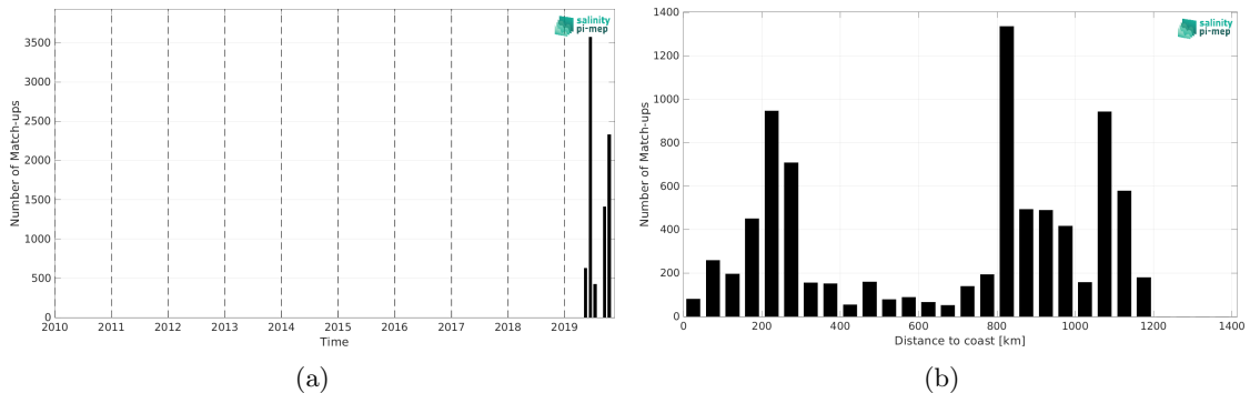
Figure 1: Number of match-ups between Saildrone and SMOS SSS L3 v2 - 9-Days (BEC) SSS as a function of time (a) and as function of the distance to coast (b) over the Gulf Stream Pi-MEP region and for the full satellite product period.
