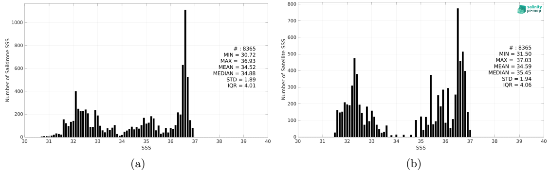
Figure 2: Histograms of SSS from Saildrone (a) and SMOS SSS L3 v2 - 9-Days (BEC) (b) considering all match-up pairs per bins of 0.1 over the Gulf Stream Pi-MEP region and for the full satellite product period.
