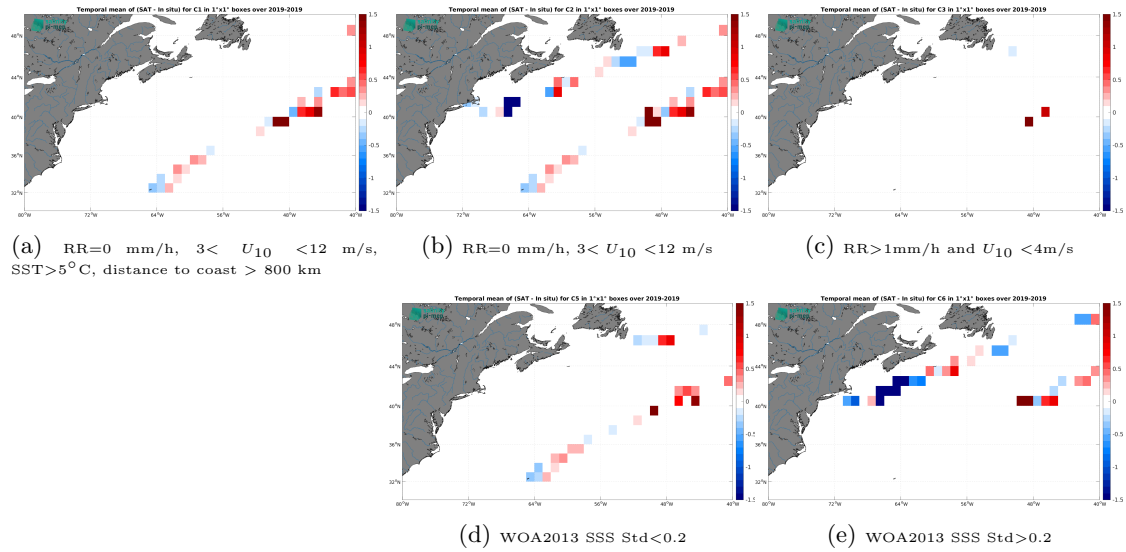
Figure 12: Temporal mean gridded over spatial boxes of size 1^\circ \times 1^\circ of \Delta SSS (SMOS SSS L3 v2 - 9-Days (BEC) - Saildrone) for 5 different subdatasets corresponding to:RR=0 mm/h, 3 < U_{10} < 12 m/s, SST >5^\circ C, distance to coast > 800 km (a), RR=0 mm/h, 3 < U_{10} < 12 m/s (b), RR >1 mm/h and U_{10} < 4 m/s (c), WOA2013 SSS Std <0.2 (d), WOA2013 SSS Std >0.2 (e).
