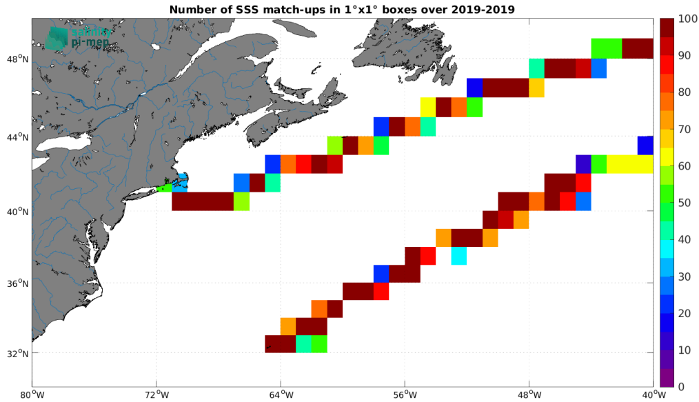
Figure 4: Number of SSS match-ups between Saildrone SSS and the SMOS SSS L3 v2 - 9-Days (BEC) SSS product for the Gulf Stream Pi-MEP region over 1^{\circ} \times 1^{\circ} boxes and for the full satellite product period.
