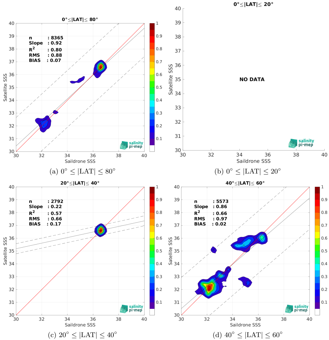
Figure 9: Contour maps of the concentration of SMOS SSS L3 v2 - 9-Days (BEC) SSS (y-axis) versus Saildrone SSS (x-axis) at match-up pairs for different latitude bands. For each plot, the red line shows x=y . The black thin and dashed lines indicate a linear fit through the data cloud and the \pm 95\% confidence levels, respectively. The number match-up pairs n , the slope and R^2 coefficient of the linear fit, the root mean square (RMS) and the mean bias between satellite and in situ data are indicated for each latitude band in each plots.
