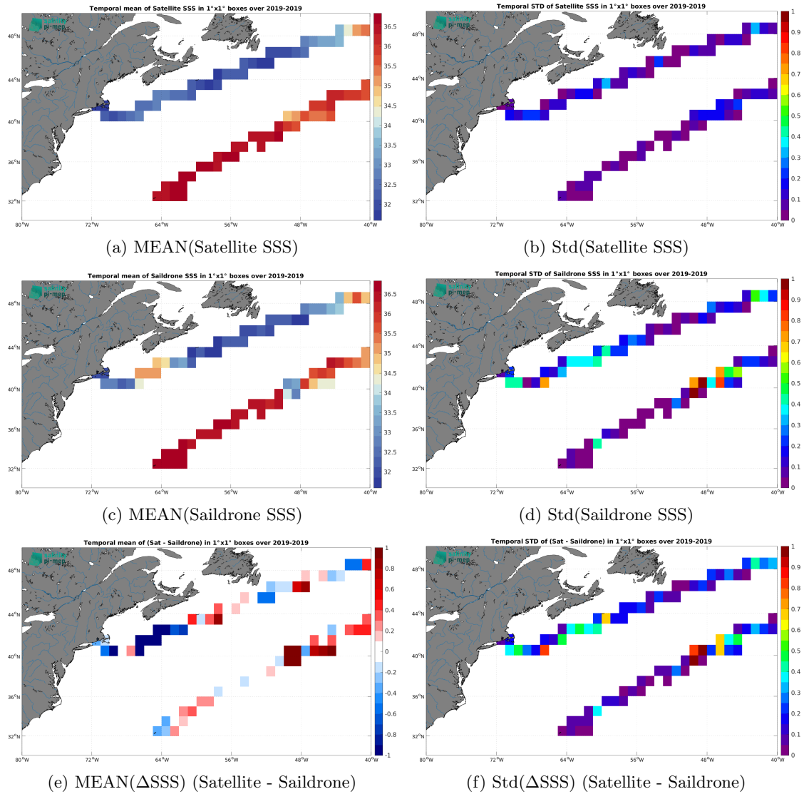
Figure 6: Temporal mean (left) and Std (right) of SSS from SMOS SSS L3 v2 - 9-Days (BEC) (top), Saildrone (middle), and of \Delta SSS (Satellite - Saildrone). Only match-up pairs are used to generate these maps.
