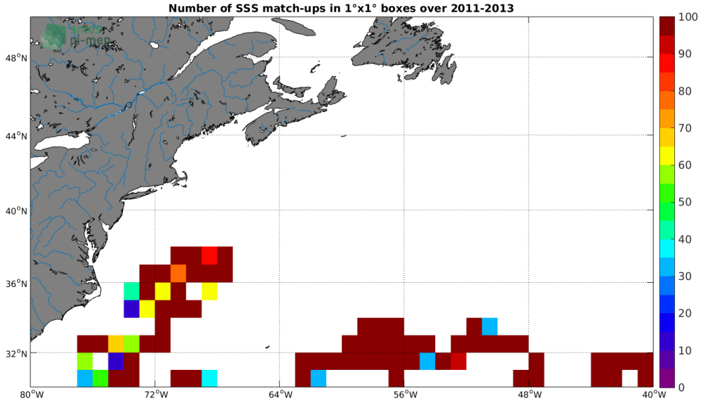
Figure 3: Number of SSS match-ups between Surface drifters SSS and the SMOS L3 v2 - 9-Days (BEC) SSS product for the Gulf Stream Pi-MEP region over 1°x1° boxes and for the full satellite product period.
