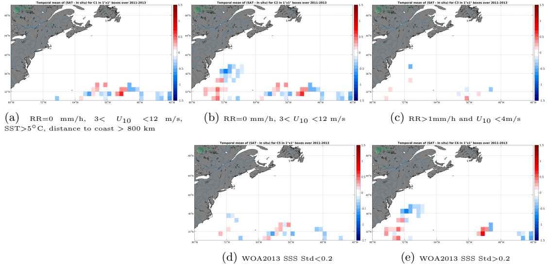
Figure 11: Temporal mean gridded over spatial boxes of size 1^{\circ}\times 1^{\circ} of \Delta\text{SSS} (SMOS L3 v2 - 9-Days (BEC) - Surface drifters) for 5 different subdatasets corresponding to:RR=0 mm/h, 3 < U_{10} < 12 m/s, SST > 5^{\circ}\text{C} , distance to coast > 800 km (a), RR=0 mm/h, 3 < U_{10} < 12 m/s (b), RR > 1 mm/h and U_{10} < 4 m/s (c), WOA2013 SSS Std < 0.2 (d), WOA2013 SSS Std > 0.2 (e).
