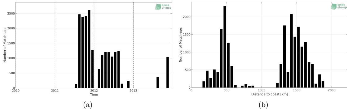
Figure 1: Number of match-ups between Surface drifters and SMOS L3 v2 - 9-Days (BEC) SSS as a function of time (a) and as function of the distance to coast (b) over the Gulf Stream Pi-MEP region and for the full satellite product period.
