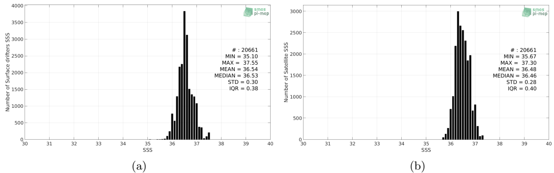
Figure 2: Histograms of SSS from Surface drifters (a) and SMOS L3 v2 - 9-Days (BEC) (b) considering all match-up pairs per bins of 0.1 over the Gulf Stream Pi-MEP region and for the full satellite product period.
