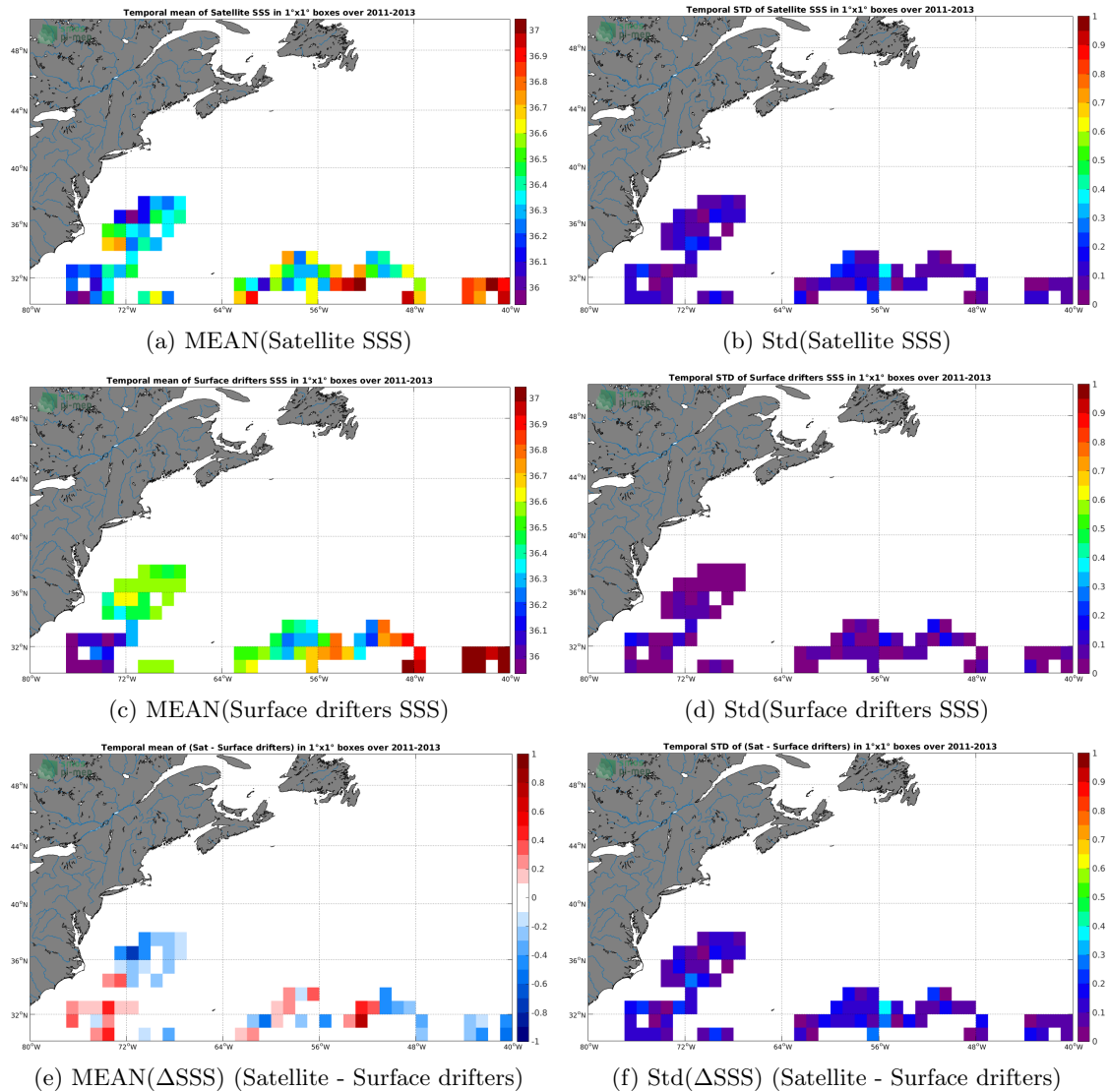
Figure 5: Temporal mean (left) and Std (right) of SSS from SMOS L3 v2 - 9-Days (BEC) (top), Surface drifters (middle), and of \Delta\text{SSS} (Satellite - Surface drifters). Only match-up pairs are used to generate these maps.
