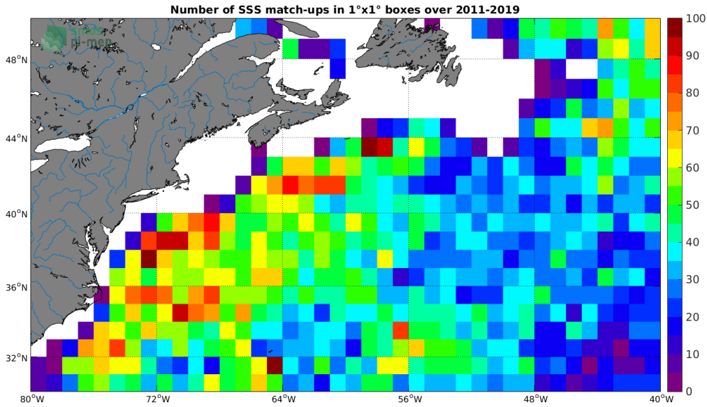
Figure 4: Number of SSS match-ups between Argo SSS and the SMOS SSS L3 v2 - 9-Days (BEC) SSS product for the Gulf Stream Pi-MEP region over 1^\circ \times 1^\circ boxes and for the full satellite product period.
