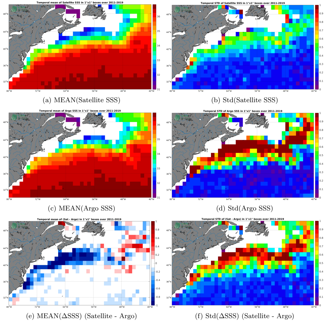
Figure 6: Temporal mean (left) and Std (right) of SSS from SMOS L3 v2 - 9-Days (BEC) (top), Argo (middle), and of \Delta SSS (Satellite - Argo). Only match-up pairs are used to generate these maps.
