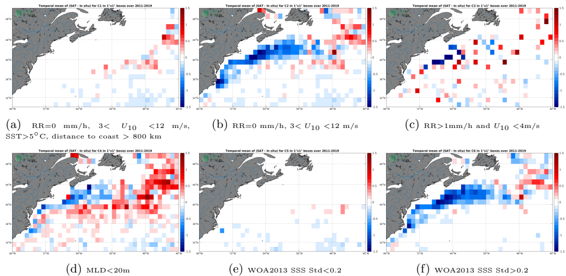
Figure 12: Temporal mean gridded over spatial boxes of size 1^\circ \times 1^\circ of \Delta SSS (SMOS L3 v2 - 9-Days (BEC) - Argo) for 6 different subdatasets corresponding to:RR=0 mm/h, 3 < U_{10} < 12 m/s, SST >5^\circ\text{C} , distance to coast > 800 km (a), RR=0 mm/h, 3 < U_{10} < 12 m/s (b), RR >1 mm/h and U_{10} < 4 m/s (c),MLD <20 m (d),WOA2013 SSS Std <0.2 (e),WOA2013 SSS Std >0.2 (f).
