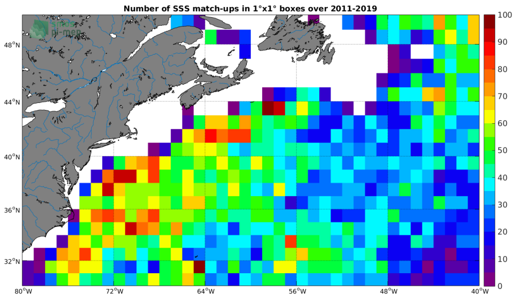
Figure 4: Number of SSS match-ups between Argos SSS and the SMOS L3 v2 - 9-Days (BEC) SSS product for the Gulf Stream Pi-MEP region over 1°x1° boxes and for the full satellite product period.
