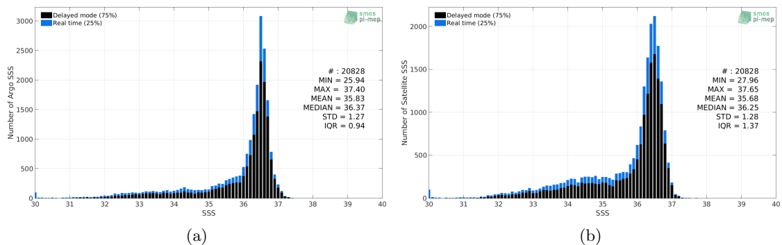
Figure 2: Histograms of SSS from Argo (a) and SMOS L3 v2 - 9-Days (BEC) (b) considering all match-up pairs per bins of 0.1 over the Gulf Stream Pi-MEP region and for the full satellite product period.
