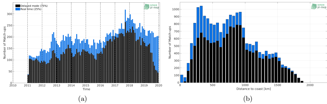
Figure 1: Number of match-ups between Argo and SMOS L3 v2 - 9-Days (BEC) SSS as a function of time (a) and as function of the distance to coast (b) over the Gulf Stream Pi-MEP region and for the full satellite product period.
