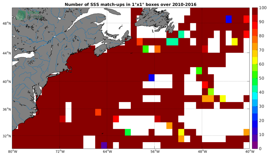
Figure 4: Number of SSS match-ups between TSG-SAMOS SSS and the SMOS-L3-BEC-OA-V1-9DAYS-0.25DEG SSS product for the Gulf Stream Pi-MEP region over 1°x1° boxes and for the full satellite product period.
