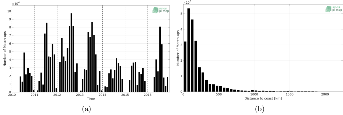
Figure 1: Number of match-ups between TSG-SAMOS and SMOS-L3-BEC-OA-V1-9DAYS-0.25DEG SSS as a function of time (a) and as function of the distance to coast (b) over the Gulf Stream Pi-MEP region and for the full satellite product period.
