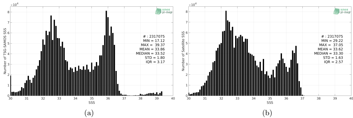
Figure 2: Histograms of SSS from TSG-SAMOS (a) and SMOS-L3-BEC-OA-V1-9DAYS-0.25DEG (b) considering all match-up pairs per bins of 0.1 over the Gulf Stream Pi-MEP region and for the full satellite product period.
