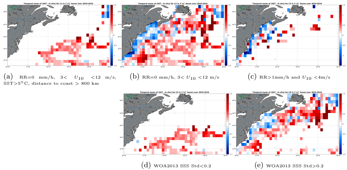
Figure 12: Temporal mean gridded over spatial boxes of size 1^\circ \times 1^\circ of \Delta SSS (SMOS-L3-BEC-OA-V1-9DAYS-0.25DEG - TSG-SAMOS) for 5 different subdatasets corresponding to:RR=0 mm/h, 3 < U_{10} < 12 m/s, SST >5^\circ C, distance to coast > 800 km (a), RR=0 mm/h, 3 < U_{10} < 12 m/s (b), RR >1 mm/h and U_{10} < 4 m/s (c), WOA2013 SSS Std <0.2 (d), WOA2013 SSS Std >0.2 (e).
