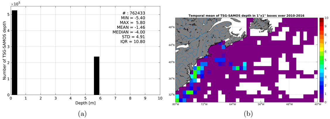
Figure 3: Histograms of the depth of the upper level SSS measurements from TSG-SAMOS in the Match-up DataBase for the Gulf Stream Pi-MEP region (a) and temporal mean spatial distribution of pressure of the in situ SSS data over 1^\circ \times 1^\circ boxes and for the full satellite product period (b).
