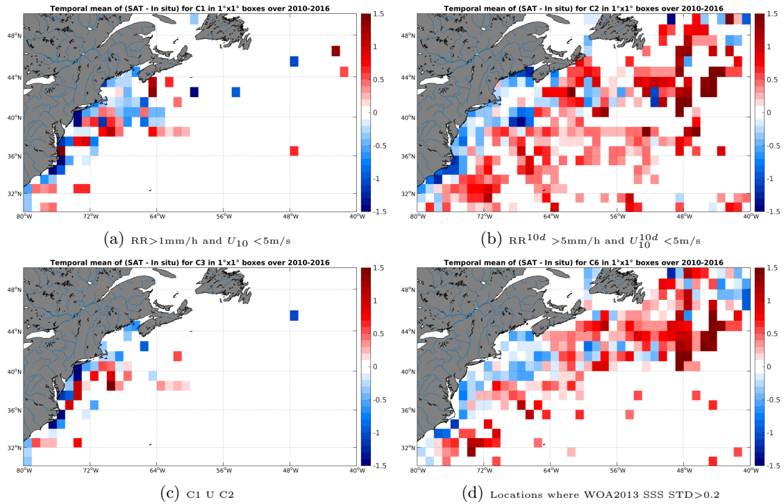
Figure 12: Temporal mean gridded over spatial boxes of size 1^\circ \times 1^\circ of \Delta SSS (SMOS-L3-BEC-OA-V1-9DAYS-0.25DEG - TSG-SAMOS) for 4 different subdatasets corresponding to:RR > 1 mm/h and U_{10} < 5 m/s (a), RR^{10d} > 5 mm/h and U_{10}^{10d} < 5 m/s (b), C1 U C2 (c),Locations where WOA2013 SSS STD > 0.2 (d).
