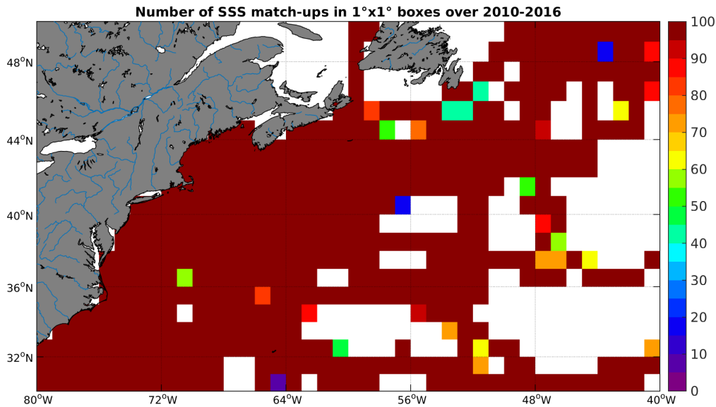
Figure 4: Number of SSS match-ups between TSG-SAMOS SSS and the SMOS-L3-BEC-OA-V1-9DAYS-0.25DEG SSS product for the Gulf Stream Pi-MEP region over 1^\circ \times 1^\circ boxes and for the full satellite product period.
