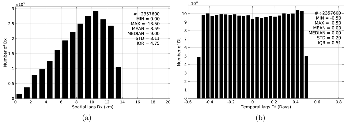
Figure 5: Histograms of the spatial (a) and temporal (b) lags between the time of the TSG-SAMOS measurements and the date of the corresponding SMOS-L3-BEC-OA-V1-9DAYS-0.25DEG SSS product.
