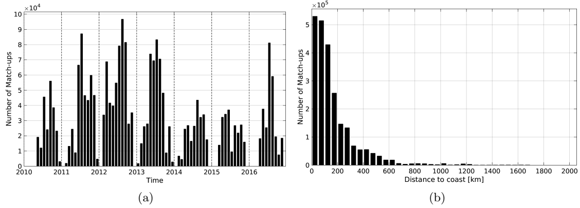
Figure 1: Number of match-ups between TSG-SAMOS and SMOS-L3-BEC-OA-V1-9DAYS-0.25DEG SSS as a function of time (a) and as function of the distance to coast (b) over the Gulf Stream Pi-MEP region and for the full satellite product period.
