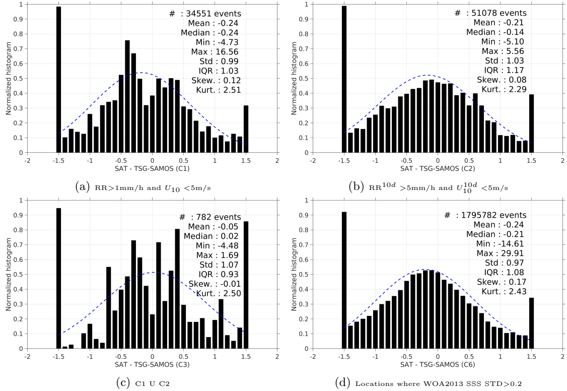
Figure 13: Normalized histogram of \Delta\text{SSS} (SMOS-L3-BEC-OA-V1-9DAYS-0.25DEG - TSG-SAMOS) for 6 different subdatasets corresponding to: RR > 1\text{mm/h} and U_{10} < 5\text{m/s} (a), RR^{10d} > 5\text{mm/h} and U_{10}^{10d} < 5\text{m/s} (b), C1 U C2 (c), Locations where WOA2013 SSS STD > 0.2 (d).
