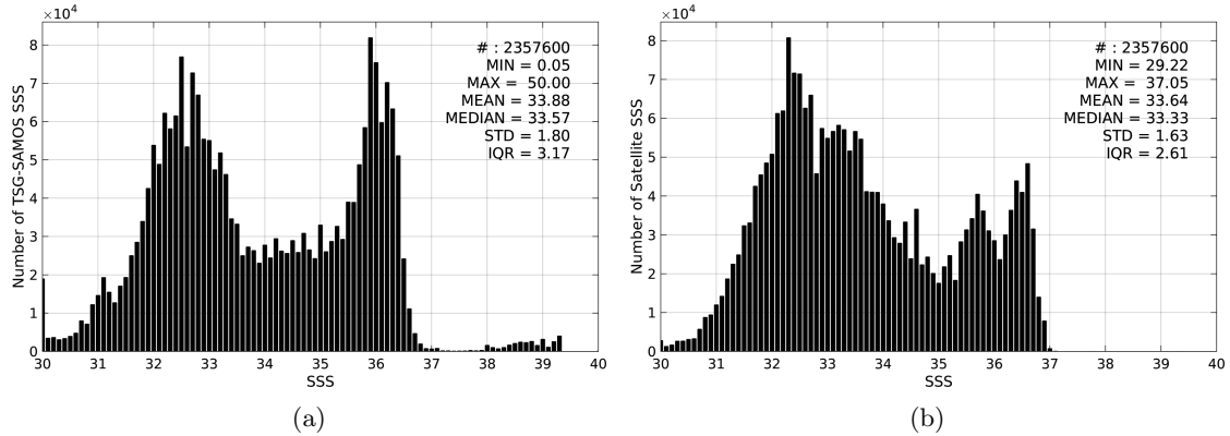
Figure 2: Histograms of SSS from TSG-SAMOS (a) and SMOS-L3-BEC-OA-V1-9DAYS-0.25DEG (b) considering all match-up pairs per bins of 0.1 over the Gulf Stream Pi-MEP region and for the full satellite product period.
