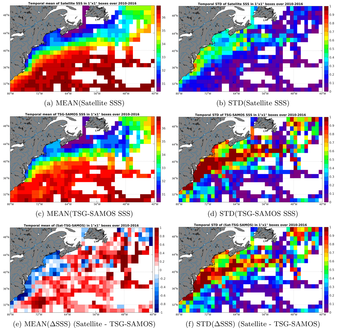
Figure 6: Temporal mean (left) and STD (right) of SSS from SMOS-L3-BEC-OA-V1-9DAYS-0.25DEG (top), TSG-SAMOS (middle), and of \Delta SSS (Satellite - TSG-SAMOS). Only match-up pairs are used to generate these maps.
