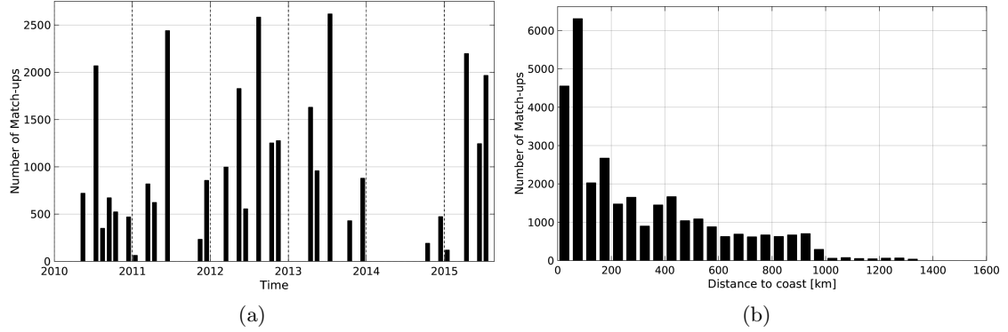
Figure 1: Number of match-ups between TSG-LEGOS-DM and SMOS-L3-BEC-OA-V1-9DAYS-0.25DEG SSS as a function of time (a) and as function of the distance to coast (b) over the Gulf Stream Pi-MEP region and for the full satellite product period.
