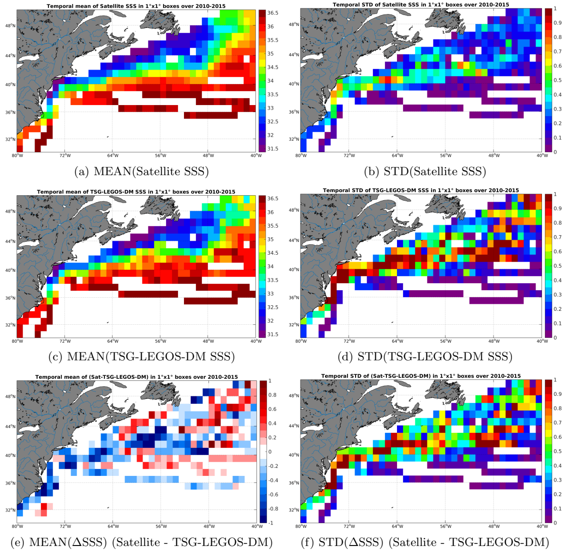
Figure 6: Temporal mean (left) and STD (right) of SSS from SMOS-L3-BEC-OA-V1-9DAYS-0.25DEG (top), TSG-LEGOS-DM (middle), and of \Delta SSS (Satellite - TSG-LEGOS-DM). Only match-up pairs are used to generate these maps.
