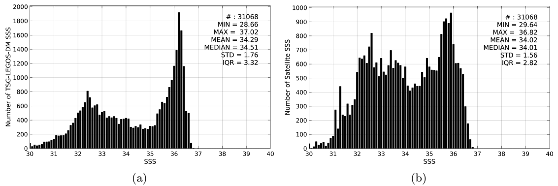
Figure 2: Histograms of SSS from TSG-LEGOS-DM (a) and SMOS-L3-BEC-OA-V1-9DAYS-0.25DEG (b) considering all match-up pairs per bins of 0.1 over the Gulf Stream Pi-MEP region and for the full satellite product period.
