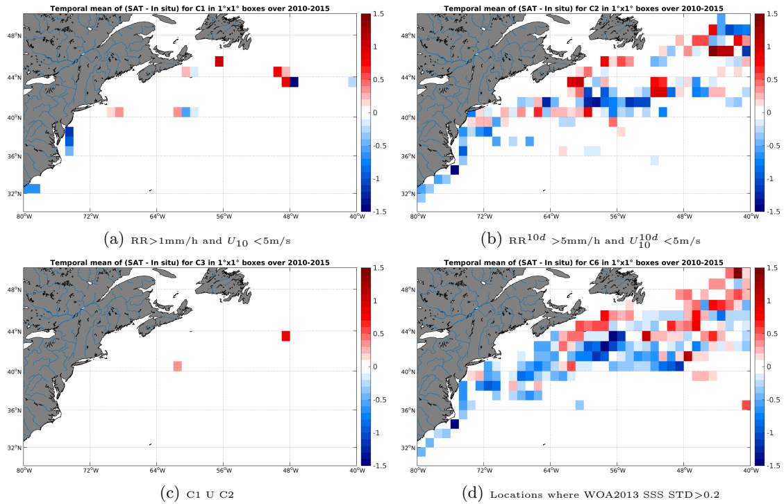
Figure 12: Temporal mean gridded over spatial boxes of size 1^\circ \times 1^\circ of \Delta SSS (SMOS-L3-BEC-OA-V1-9DAYS-0.25DEG - TSG-LEGOS-DM) for 4 different subdatasets corresponding to: RR > 1\text{mm/h} and U_{10} < 5\text{m/s} (a), RR^{10d} > 5\text{mm/h} and U_{10}^{10d} < 5\text{m/s} (b), C1 U C2 (c), Locations where WOA2013 SSS STD > 0.2 (d).
