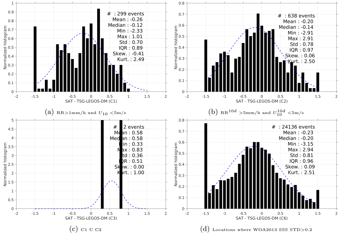
Figure 13: Normalized histogram of \Delta\text{SSS} (SMOS-L3-BEC-OA-V1-9DAYS-0.25DEG - TSG-LEGOS-DM) for 6 different subdatasets corresponding to: \text{RR} > 1\text{mm/h} and U_{10} < 5\text{m/s} (a), \text{RR}^{10d} > 5\text{mm/h} and U_{10}^{10d} < 5\text{m/s} (b), C1 U C2 (c), Locations where WOA2013 SSS STD > 0.2 (d).
