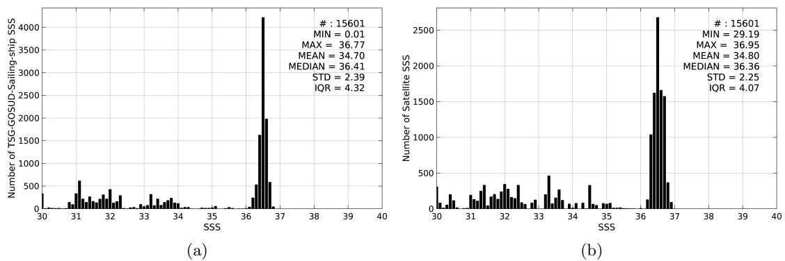
Figure 2: Histograms of SSS from TSG-GOSUD-Sailing-ship (a) and SMOS-L3-BEC-OA-V1-9DAYS-0.25DEG (b) considering all match-up pairs per bins of 0.1 over the Gulf Stream Pi-MEP region and for the full satellite product period.
