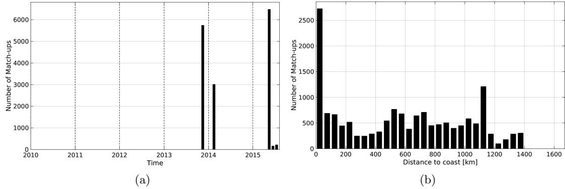
Figure 1: Number of match-ups between TSG-GOSUD-Sailing-ship and SMOS-L3-BEC-OA-V1-9DAYS-0.25DEG SSS as a function of time (a) and as function of the distance to coast (b) over the Gulf Stream Pi-MEP region and for the full satellite product period.
