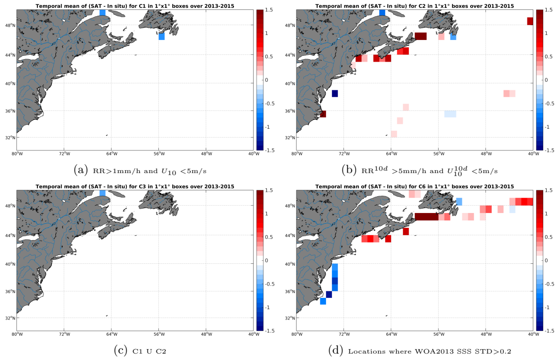
Figure 12: Temporal mean gridded over spatial boxes of size 1^\circ \times 1^\circ of \Delta SSS (SMOS-L3-BEC-OA-V1-9DAYS-0.25DEG - TSG-GOSUD-Sailing-ship) for 4 different subdatasets corresponding to: RR > 1mm/h and U_{10} < 5 m/s (a), RR^{10d} > 5 mm/h and U_{10}^{10d} < 5 m/s (b), C1 U C2 (c), Locations where WOA2013 SSS STD > 0.2 (d).
