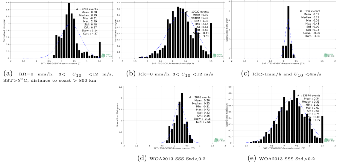
Figure 13: Normalized histogram of \Delta SSS (SMOS-L3-BEC-OA-V1-9DAYS-0.25DEG - TSG-GOSUD-Research-vessel) for 5 different subdatasets corresponding to: RR=0 mm/h, 3 < U_{10} < 12 m/s, SST>5°C, distance to coast > 800 km (a), RR=0 mm/h, 3 < U_{10} < 12 m/s (b), RR>1mm/h and U_{10} < 4 m/s (c), WOA2013 SSS Std<0.2 (d), WOA2013 SSS Std>0.2 (e).
