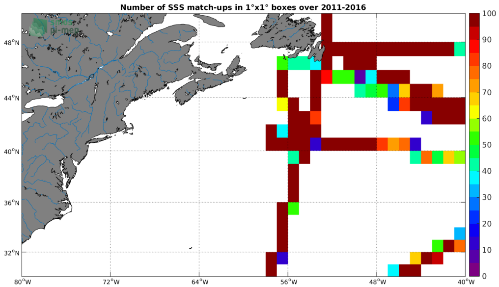
Figure 4: Number of SSS match-ups between TSG-GOSUD-Research-vessel SSS and the SMOS-L3-BEC-OA-V1-9DAYS-0.25DEG SSS product for the Gulf Stream Pi-MEP region over 1°x1° boxes and for the full satellite product period.
