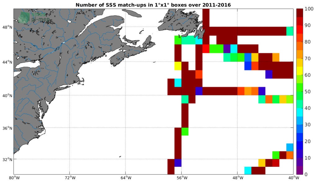
Figure 4: Number of SSS match-ups between TSG-GOSUD-Research-vessel SSS and the SMOS-L3-BEC-OA-V1-9DAYS-0.25DEG SSS product for the Gulf Stream Pi-MEP region over 1^\circ \times 1^\circ boxes and for the full satellite product period.
