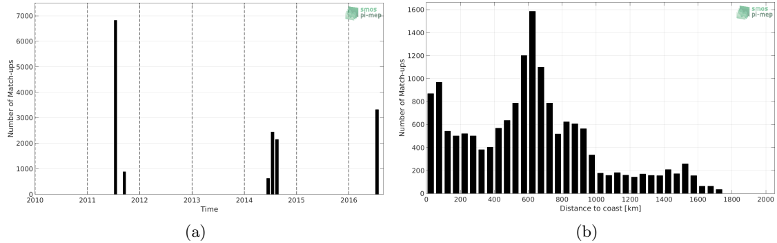
Figure 1: Number of match-ups between TSG-GOSUD-Research-vessel and SMOS-L3-BEC-OA-V1-9DAYS-0.25DEG SSS as a function of time (a) and as function of the distance to coast (b) over the Gulf Stream Pi-MEP region and for the full satellite product period.
