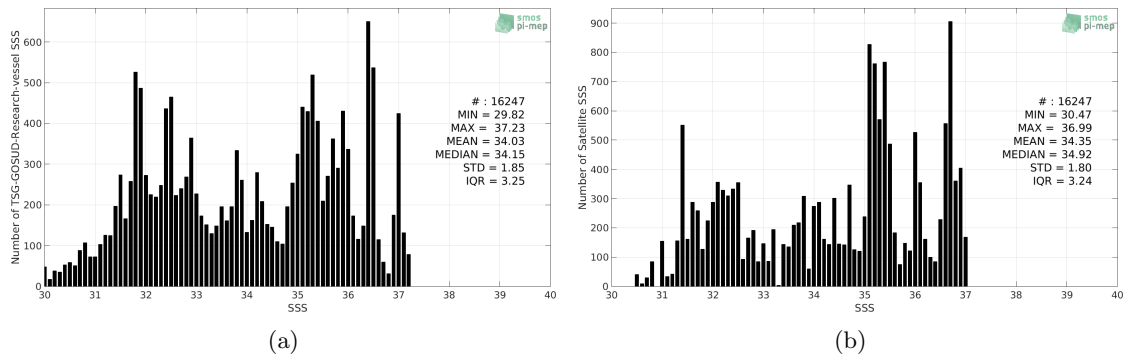
Figure 2: Histograms of SSS from TSG-GOSUD-Research-vessel (a) and SMOS-L3-BEC-OA-V1-9DAYS-0.25DEG (b) considering all match-up pairs per bins of 0.1 over the Gulf Stream Pi-MEP region and for the full satellite product period.
