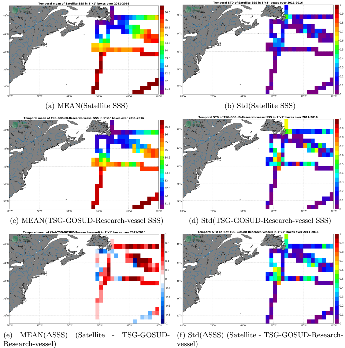
Figure 6: Temporal mean (left) and Std (right) of SSS from SMOS-L3-BEC-OA-V1-9DAYS-0.25DEG (top), TSG-GOSUD-Research-vessel (middle), and of \Delta SSS (Satellite - TSG-GOSUD-Research-vessel). Only match-up pairs are used to generate these maps.
