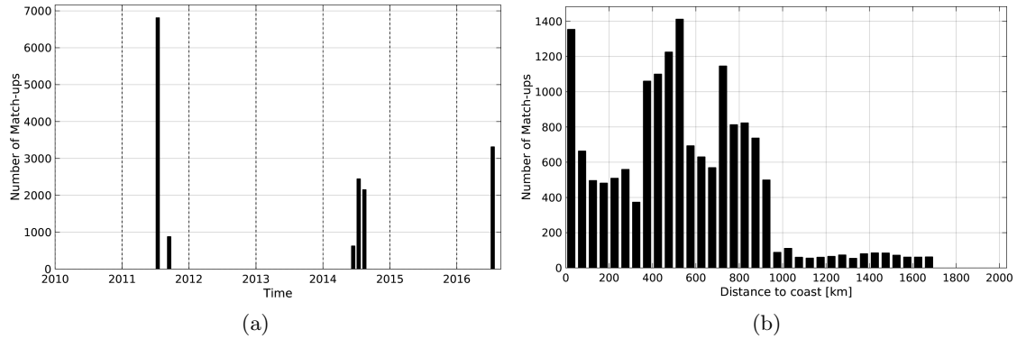
Figure 1: Number of match-ups between TSG-GOSUD-Research-vessel and SMOS-L3-BEC-OA-V1-9DAYS-0.25DEG SSS as a function of time (a) and as function of the distance to coast (b) over the Gulf Stream Pi-MEP region and for the full satellite product period.
