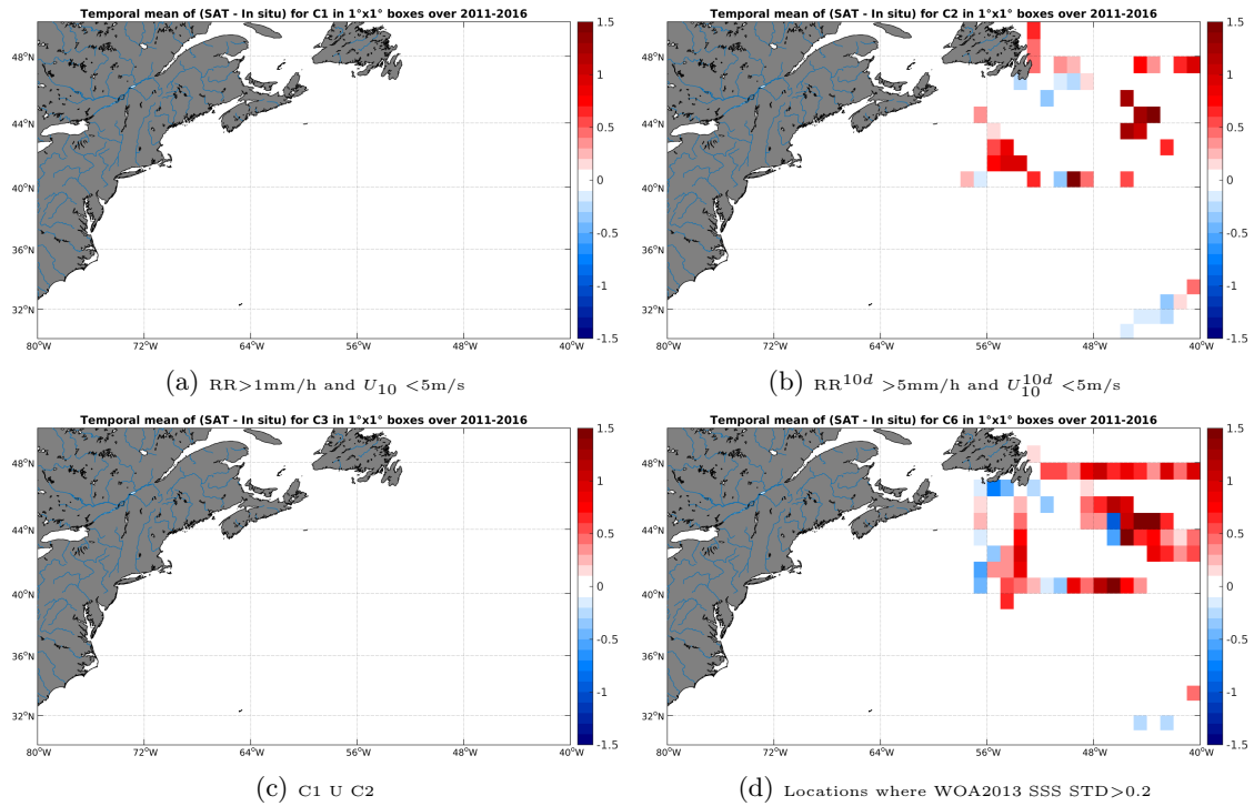
Figure 12: Temporal mean gridded over spatial boxes of size 1^\circ \times 1^\circ of \Delta SSS (SMOS-L3-BEC-OA-V1-9DAYS-0.25DEG - TSG-GOSUD-Research-vessel) for 4 different subdatasets corresponding to: RR > 1mm/h and U_{10} < 5m/s (a), RR^{10d} > 5mm/h and U_{10}^{10d} < 5m/s (b), C1 U C2 (c), Locations where WOA2013 SSS STD > 0.2 (d).
