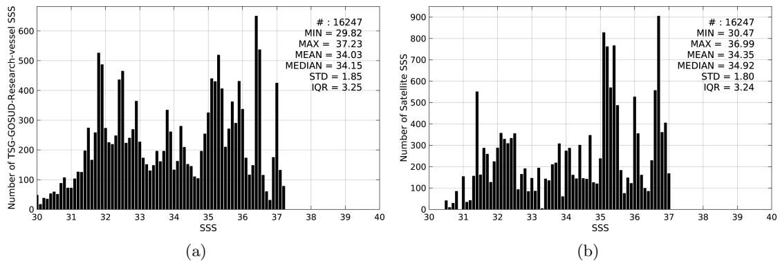
Figure 2: Histograms of SSS from TSG-GOSUD-Research-vessel (a) and SMOS-L3-BEC-OA-V1-9DAYS-0.25DEG (b) considering all match-up pairs per bins of 0.1 over the Gulf Stream Pi-MEP region and for the full satellite product period.
