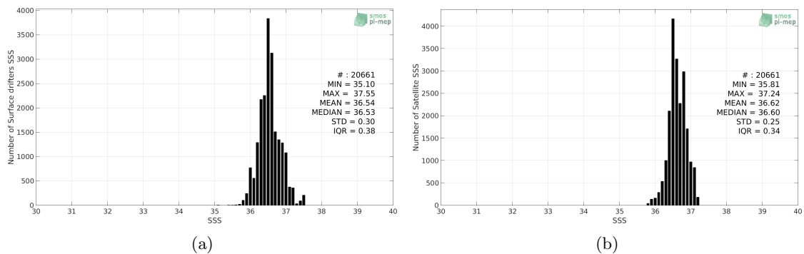
Figure 2: Histograms of SSS from Surface drifters (a) and SMOS-L3-BEC-OA-V1-9DAYS-0.25DEG (b) considering all match-up pairs per bins of 0.1 over the Gulf Stream Pi-MEP region and for the full satellite product period.
