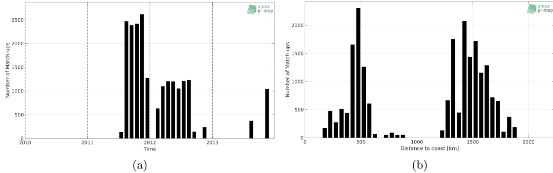
Figure 1: Number of match-ups between Surface drifters and SMOS-L3-BEC-OA-V1-9DAYS-0.25DEG SSS as a function of time (a) and as function of the distance to coast (b) over the Gulf Stream Pi-MEP region and for the full satellite product period.
