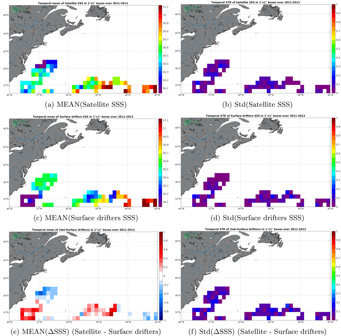
Figure 5: Temporal mean (left) and Std (right) of SSS from SMOS-L3-BEC-OA-V1-9DAYS-0.25DEG (top), Surface drifters (middle), and of \Delta\text{SSS} (Satellite - Surface drifters). Only match-up pairs are used to generate these maps.
