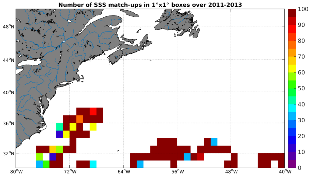
Figure 3: Number of SSS match-ups between Surface drifters SSS and the SMOS-L3-BEC-OA-V1-9DAYS-0.25DEG SSS product for the Gulf Stream Pi-MEP region over 1^\circ \times 1^\circ boxes and for the full satellite product period.
