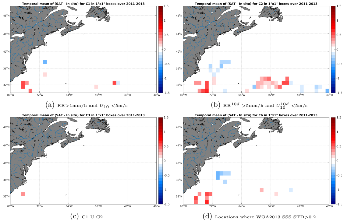
Figure 11: Temporal mean gridded over spatial boxes of size 1^\circ \times 1^\circ of \Delta SSS (SMOS-L3-BEC-OA-V1-9DAYS-0.25DEG - Surface drifters) for 4 different subdatasets corresponding to:RR > 1mm/h and U_{10} < 5 m/s (a), RR^{10d} > 5 mm/h and U_{10}^{10d} < 5 m/s (b), C1 U C2 (c),Locations where WOA2013 SSS STD > 0.2 (d).
