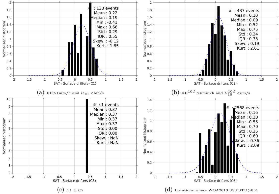
Figure 12: Normalized histogram of \Delta\text{SSS} (SMOS-L3-BEC-OA-V1-9DAYS-0.25DEG - Surface drifters) for 6 different subdatasets corresponding to: RR > 1\text{mm/h} and U_{10} < 5\text{m/s} (a), RR^{10d} > 5\text{mm/h} and U_{10}^{10d} < 5\text{m/s} (b), C1 U C2 (c), Locations where WOA2013 SSS STD > 0.2 (d).
