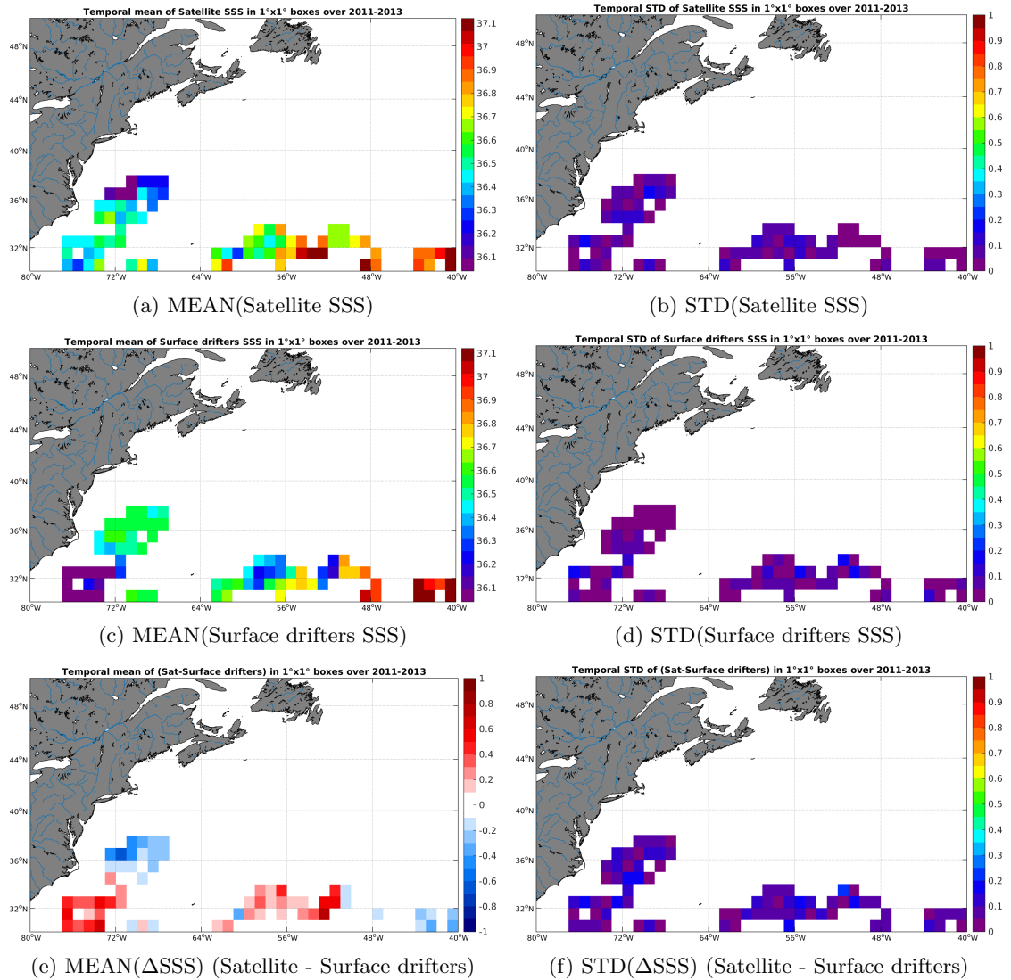
Figure 5: Temporal mean (left) and STD (right) of SSS from SMOS-L3-BEC-OA-V1-9DAYS-0.25DEG (top), Surface drifters (middle), and of \Delta SSS (Satellite - Surface drifters). Only match-up pairs are used to generate these maps.
