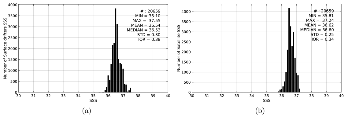
Figure 2: Histograms of SSS from Surface drifters (a) and SMOS-L3-BEC-OA-V1-9DAYS-0.25DEG (b) considering all match-up pairs per bins of 0.1 over the Gulf Stream Pi-MEP region and for the full satellite product period.
