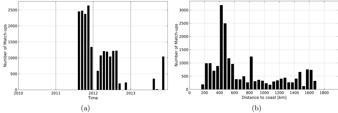
Figure 1: Number of match-ups between Surface drifters and SMOS-L3-BEC-OA-V1-9DAYS-0.25DEG SSS as a function of time (a) and as function of the distance to coast (b) over the Gulf Stream Pi-MEP region and for the full satellite product period.
