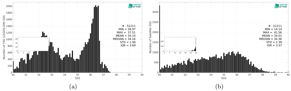
Figure 3: Histograms of SSS from TSG (LEGOS-DM) (a) and SMOS SSS L2 v700 (ESA) (b) considering all match-up pairs per bins of 0.1 over the Gulf Stream Pi-MEP region and for the full satellite product period.
