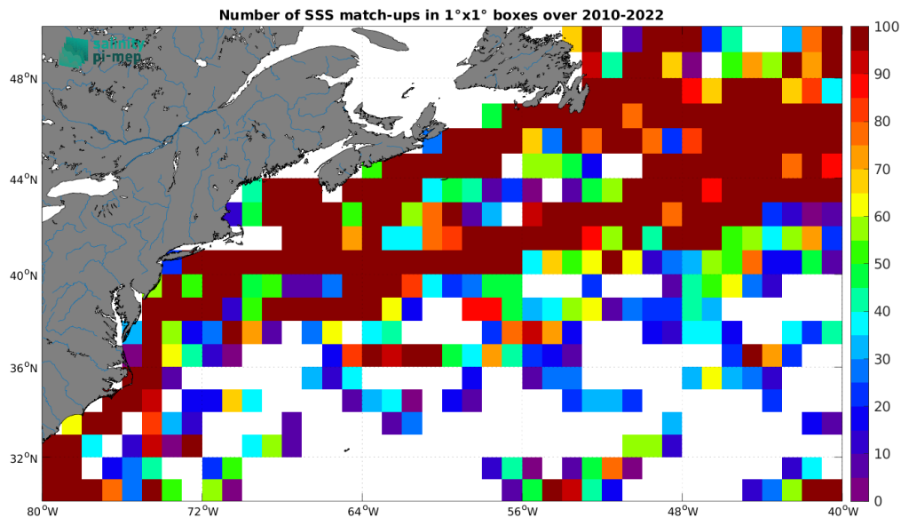
Figure 5: Number of SSS match-ups between TSG (LEGOS-DM) SSS and the SMOS SSS L2 v700 (ESA) SSS product for the Gulf Stream Pi-MEP region over 1^\circ \times 1^\circ boxes and for the full satellite product period.
