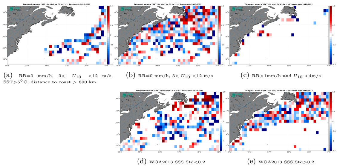
Figure 14: Temporal mean gridded over spatial boxes of size 1^\circ \times 1^\circ of \Delta SSS (SMOS SSS L2 v700 (ESA) - TSG (LEGOS-DM)) for 5 different subdatasets corresponding to:RR=0 mm/h, 3 < U_{10} < 12 m/s, SST>5°C, distance to coast > 800 km (a), RR=0 mm/h, 3 < U_{10} < 12 m/s (b), RR>1mm/h and U_{10} < 4 m/s (c), WOA2013 SSS Std<0.2 (d), WOA2013 SSS Std>0.2 (e).
