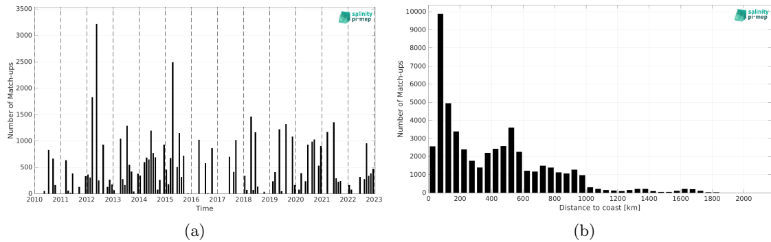
Figure 2: Number of match-ups between TSG (LEGOS-DM) and SMOS SSS L2 v700 (ESA) SSS as a function of time (a) and as function of the distance to coast (b) over the Gulf Stream Pi-MEP region and for the full satellite product period.
