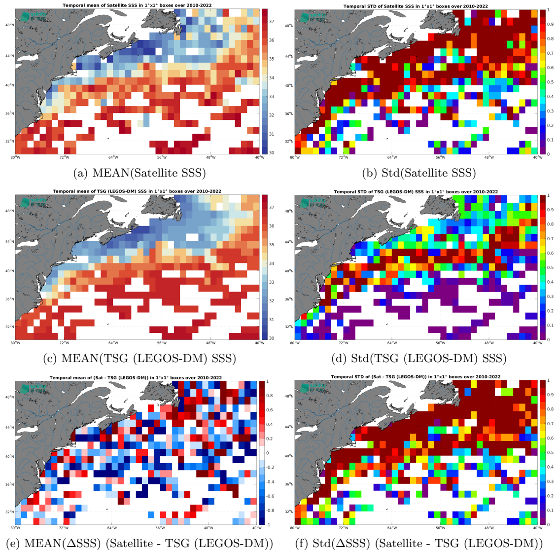
Figure 7: Temporal mean (left) and Std (right) of SSS from SMOS SSS L2 v700 (ESA) (top), TSG (LEGOS-DM) (middle), and of \Delta SSS (Satellite - TSG (LEGOS-DM)). Only match-up pairs are used to generate these maps.
