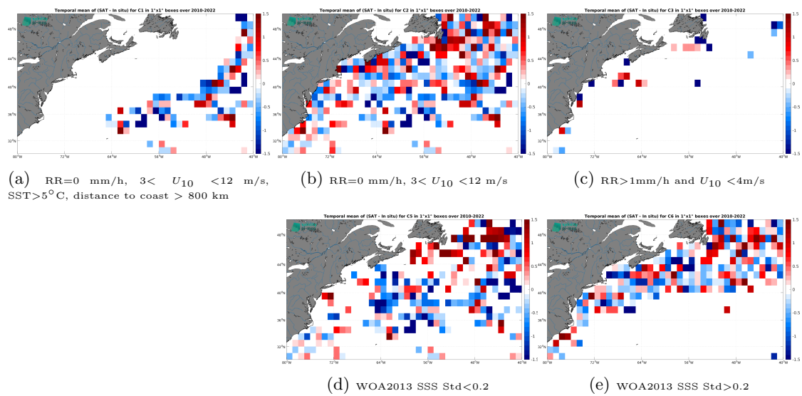
Figure 14: Temporal mean gridded over spatial boxes of size 1^\circ \times 1^\circ of \Delta SSS (SMOS SSS L2 v700 (ESA) - TSG (LEGOS-DM)) for 5 different subdatasets corresponding to: RR=0 mm/h, 3 < U_{10} < 12 m/s, SST > 5°C, distance to coast > 800 km (a), RR=0 mm/h, 3 < U_{10} < 12 m/s (b), RR > 1mm/h and U_{10} < 4 m/s (c), WOA2013 SSS Std < 0.2 (d), WOA2013 SSS Std > 0.2 (e).
