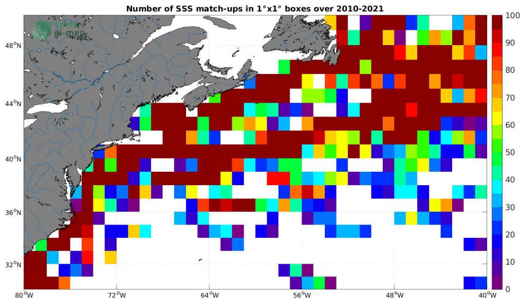
Figure 4: Number of SSS match-ups between TSG (LEGOS-DM) SSS and the SMOS SSS L2 v700 (ESA) SSS product for the Gulf Stream Pi-MEP region over 1^\circ \times 1^\circ boxes and for the full satellite product period.
