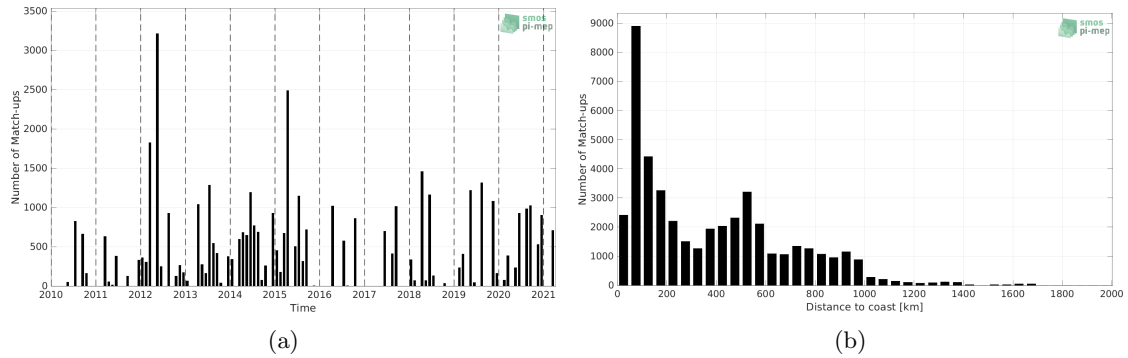
Figure 1: Number of match-ups between TSG (LEGOS-DM) and SMOS SSS L2 v700 (ESA) SSS as a function of time (a) and as function of the distance to coast (b) over the Gulf Stream Pi-MEP region and for the full satellite product period.
