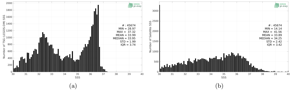
Figure 2: Histograms of SSS from TSG (LEGOS-DM) (a) and SMOS SSS L2 v700 (ESA) (b) considering all match-up pairs per bins of 0.1 over the Gulf Stream Pi-MEP region and for the full satellite product period.
