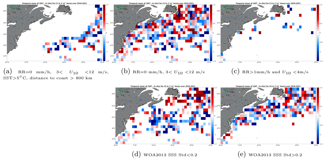
Figure 12: Temporal mean gridded over spatial boxes of size 1^\circ \times 1^\circ of \Delta SSS (SMOS SSS L2 v700 (ESA) - TSG (LEGOS-DM)) for 5 different subdatasets corresponding to:RR=0 mm/h, 3 < U_{10} < 12 m/s, SST >5^\circ C, distance to coast > 800 km (a), RR=0 mm/h, 3 < U_{10} < 12 m/s (b), RR >1 mm/h and U_{10} < 4 m/s (c), WOA2013 SSS Std <0.2 (d), WOA2013 SSS Std >0.2 (e).
