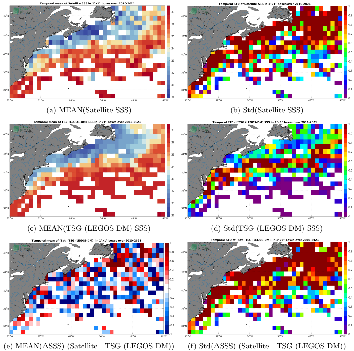
Figure 6: Temporal mean (left) and Std (right) of SSS from SMOS SSS L2 v700 (ESA) (top), TSG (LEGOS-DM) (middle), and of \Delta SSS (Satellite - TSG (LEGOS-DM)). Only match-up pairs are used to generate these maps.
