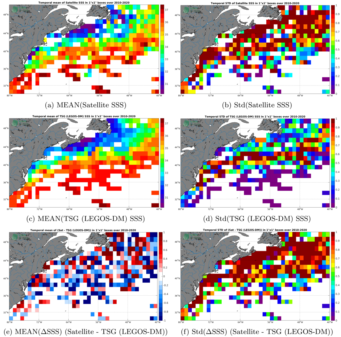
Figure 6: Temporal mean (left) and Std (right) of SSS from SMOS SSS L2 v700 (ESA) (top), TSG (LEGOS-DM) in situ dataset (middle), and of \Delta SSS (Satellite - TSG (LEGOS-DM)). Only match-up pairs are used to generate these maps.
