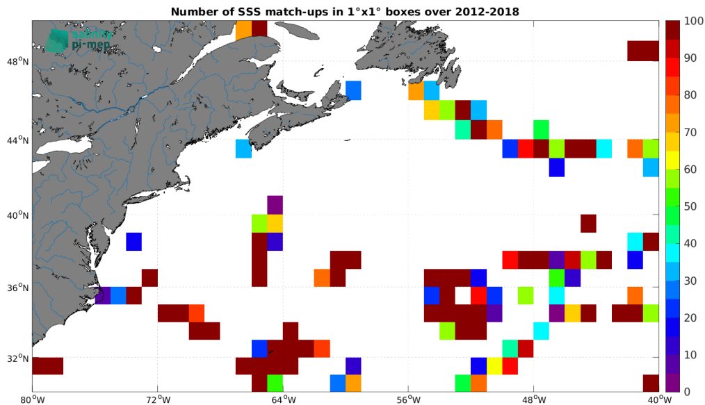
Figure 4: Number of SSS match-ups between TSG (GOSUD-Sailing-ship) SSS and the SMOS SSS L2 v700 (ESA) SSS product for the Gulf Stream Pi-MEP region over 1^\circ \times 1^\circ boxes and for the full satellite product period.
