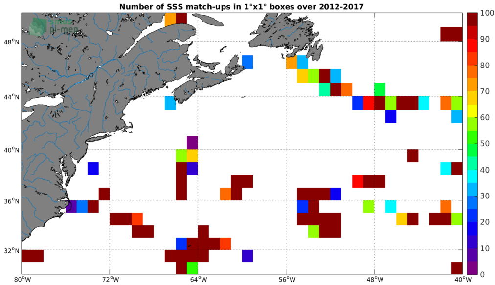
Figure 4: Number of SSS match-ups between TSG (GOSUD-Sailing-ship) SSS and the SMOS SSS L2 v700 (ESA) SSS product for the Gulf Stream Pi-MEP region over 1^{\circ} \times 1^{\circ} boxes and for the full satellite product period.
