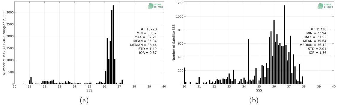
Figure 2: Histograms of SSS from TSG (GOSUD-Sailing-ship) (a) and SMOS SSS L2 v700 (ESA) (b) considering all match-up pairs per bins of 0.1 over the Gulf Stream Pi-MEP region and for the full satellite product period.
