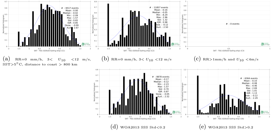
Figure 13: Normalized histogram of \Delta SSS (SMOS SSS L2 v700 (ESA) - TSG (GOSUD-Sailing-ship)) for 5 different subdatasets corresponding to: RR=0 mm/h, 3 < U_{10} < 12 m/s, SST > 5°C, distance to coast > 800 km (a), RR=0 mm/h, 3 < U_{10} < 12 m/s (b), RR > 1mm/h and U_{10} < 4 m/s (c), WOA2013 SSS Std < 0.2 (d), WOA2013 SSS Std > 0.2 (e).
