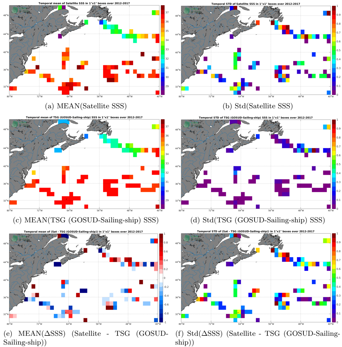
Figure 6: Temporal mean (left) and Std (right) of SSS from SMOS SSS L2 v700 (ESA) (top), TSG (GOSUD-Sailing-ship) (middle), and of \Delta SSS (Satellite - TSG (GOSUD-Sailing-ship)). Only match-up pairs are used to generate these maps.
