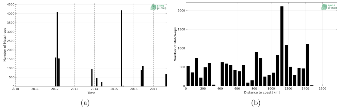
Figure 1: Number of match-ups between TSG (GOSUD-Sailing-ship) and SMOS SSS L2 v700 (ESA) SSS as a function of time (a) and as function of the distance to coast (b) over the Gulf Stream Pi-MEP region and for the full satellite product period.
