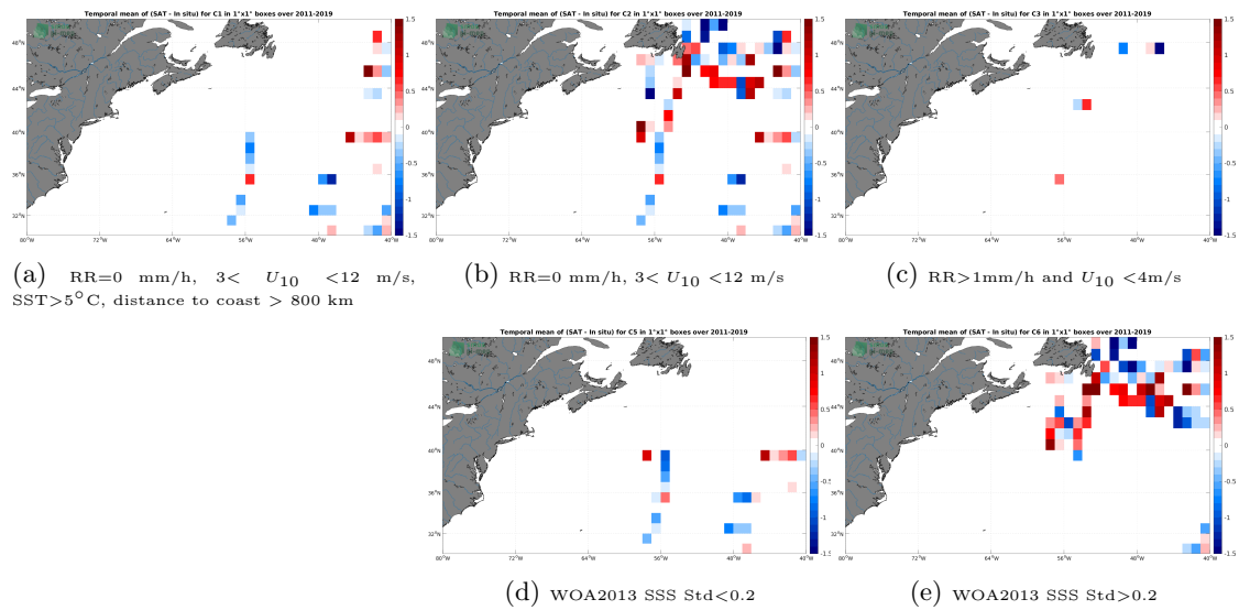
Figure 12: Temporal mean gridded over spatial boxes of size 1^\circ \times 1^\circ of \Delta SSS (SMOS SSS L2 v700 (ESA) - TSG (GOSUD-Research-vessel)) for 5 different subdatasets corresponding to:RR=0 mm/h, 3 < U_{10} < 12 m/s, SST>5°C, distance to coast > 800 km (a), RR=0 mm/h, 3 < U_{10} < 12 m/s (b), RR>1mm/h and U_{10} < 4 m/s (c), WOA2013 SSS Std<0.2 (d), WOA2013 SSS Std>0.2 (e).
