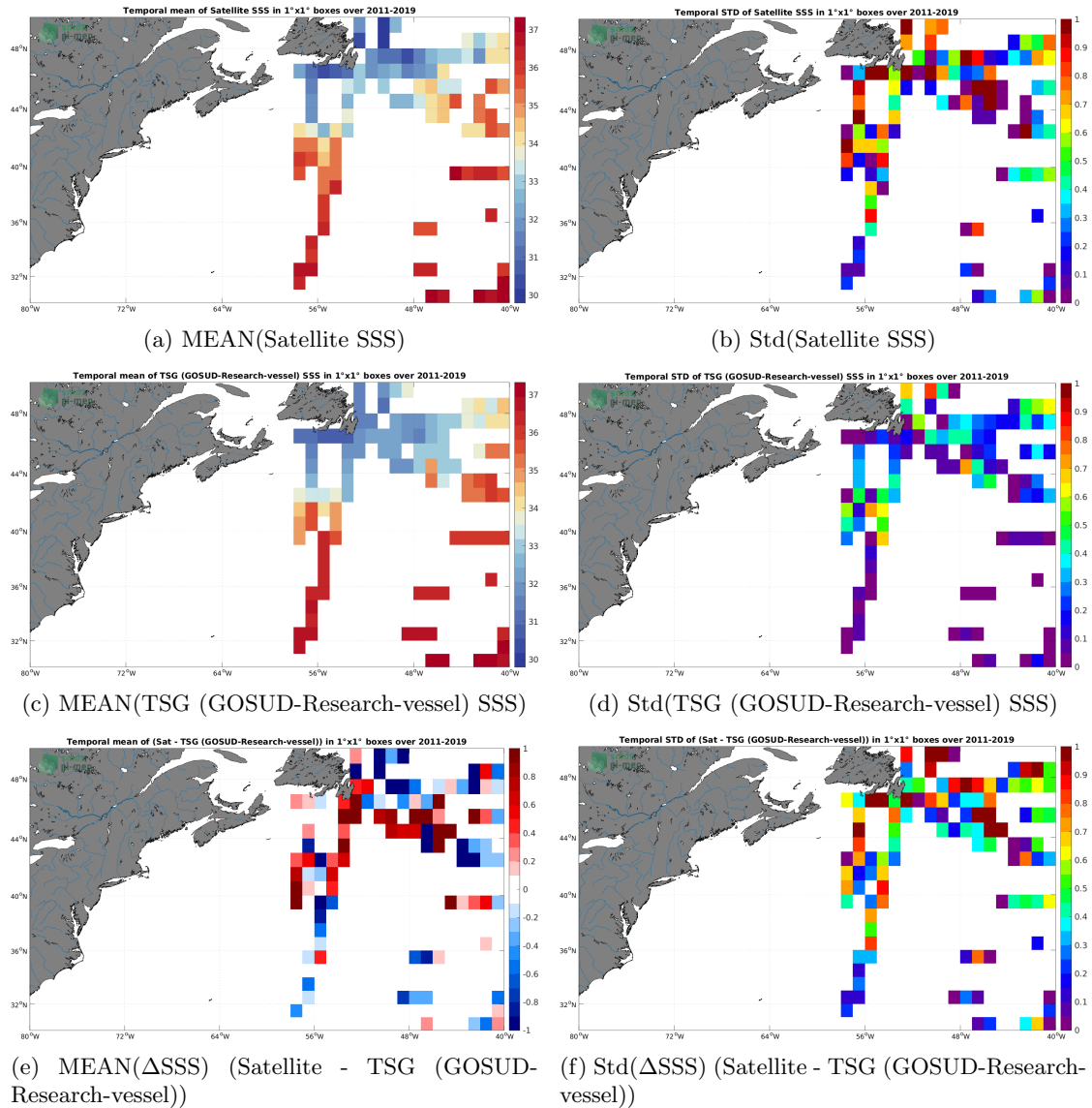
Figure 6: Temporal mean (left) and Std (right) of SSS from SMOS SSS L2 v700 (ESA) (top), TSG (GOSUD-Research-vessel) (middle), and of \Delta SSS (Satellite - TSG (GOSUD-Research-vessel)). Only match-up pairs are used to generate these maps.
