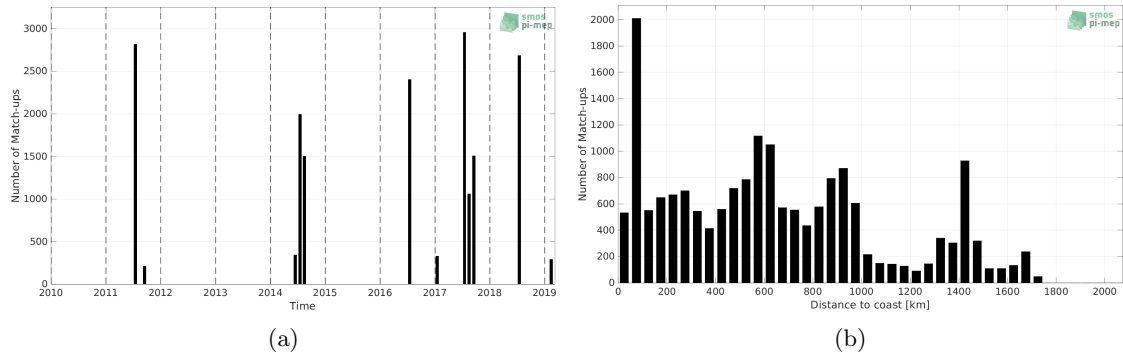
Figure 1: Number of match-ups between TSG (GOSUD-Research-vessel) and SMOS SSS L2 v700 (ESA) SSS as a function of time (a) and as function of the distance to coast (b) over the Gulf Stream Pi-MEP region and for the full satellite product period.
