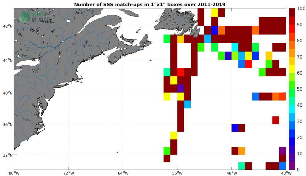
Figure 4: Number of SSS match-ups between TSG (GOSUD-Research-vessel) SSS and the SMOS SSS L2 v700 (ESA) SSS product for the Gulf Stream Pi-MEP region over 1^\circ \times 1^\circ boxes and for the full satellite product period.
