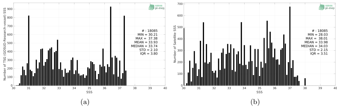
Figure 2: Histograms of SSS from TSG (GOSUD-Research-vessel) (a) and SMOS SSS L2 v700 (ESA) (b) considering all match-up pairs per bins of 0.1 over the Gulf Stream Pi-MEP region and for the full satellite product period.
