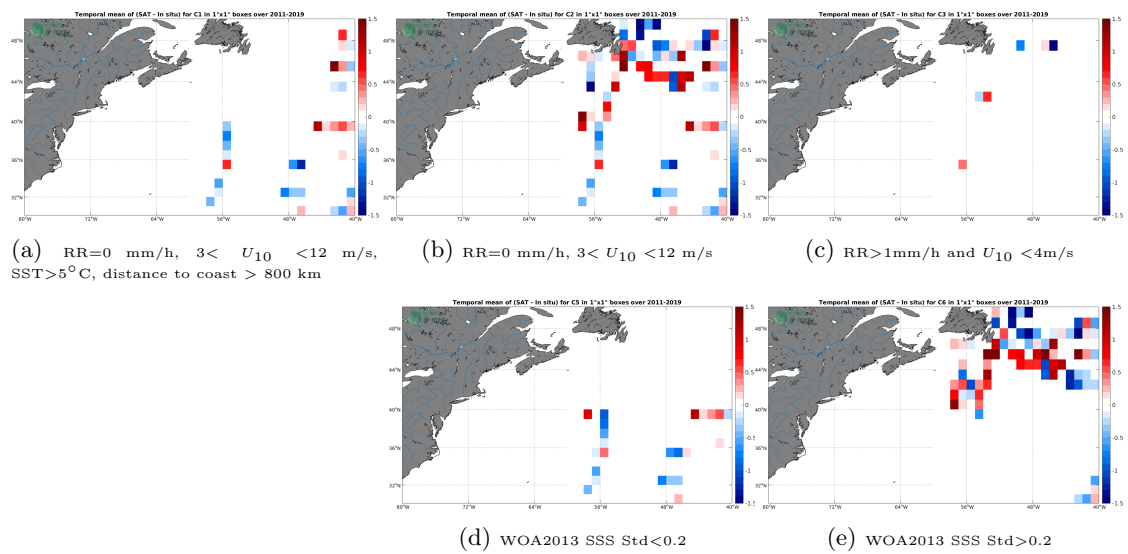
Figure 12: Temporal mean gridded over spatial boxes of size 1^\circ \times 1^\circ of \Delta\text{SSS} (SMOS SSS L2 v700 (ESA) - TSG (GOSUD-Research-vessel)) for 5 different subdatasets corresponding to: RR=0 mm/h, 3 < U_{10} < 12 m/s, SST > 5°C, distance to coast > 800 km (a), RR=0 mm/h, 3 < U_{10} < 12 m/s (b), RR > 1mm/h and U_{10} < 4 m/s (c), WOA2013 SSS Std < 0.2 (d), WOA2013 SSS Std > 0.2 (e).
