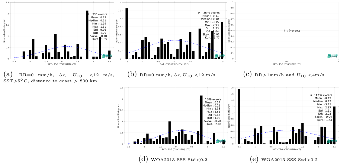
Figure 15: Normalized histogram of \Delta SSS (SMOS SSS L2 v700 (ESA) - TSG (CSIC-UTM)) for 5 different subdatasets corresponding to: RR=0 mm/h, 3 < U_{10} < 12 m/s, SST > 5°C, distance to coast > 800 km (a), RR=0 mm/h, 3 < U_{10} < 12 m/s (b), RR > 1mm/h and U_{10} < 4 m/s (c), WOA2013 SSS Std < 0.2 (d), WOA2013 SSS Std > 0.2 (e).
