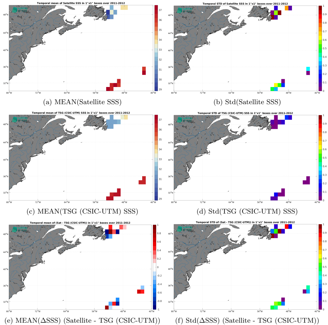
Figure 7: Temporal mean (left) and Std (right) of SSS from SMOS SSS L2 v700 (ESA) (top), TSG (CSIC-UTM) (middle), and of \Delta SSS (Satellite - TSG (CSIC-UTM)). Only match-up pairs are used to generate these maps.
