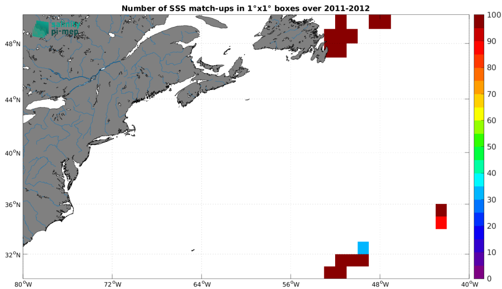
Figure 5: Number of SSS match-ups between TSG (CSIC-UTM) SSS and the SMOS SSS L2 v700 (ESA) SSS product for the Gulf Stream Pi-MEP region over 1^\circ \times 1^\circ boxes and for the full satellite product period.
