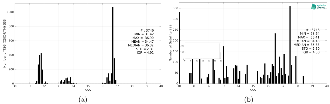
Figure 3: Histograms of SSS from TSG (CSIC-UTM) (a) and SMOS SSS L2 v700 (ESA) (b) considering all match-up pairs per bins of 0.1 over the Gulf Stream Pi-MEP region and for the full satellite product period.
