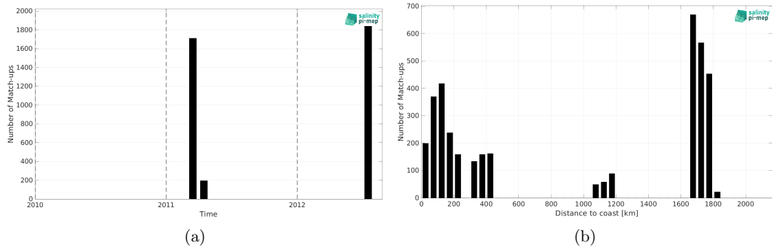
Figure 2: Number of match-ups between TSG (CSIC-UTM) and SMOS SSS L2 v700 (ESA) SSS as a function of time (a) and as function of the distance to coast (b) over the Gulf Stream Pi-MEP region and for the full satellite product period.
