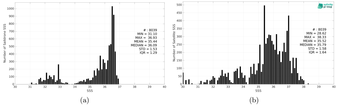
Figure 2: Histograms of SSS from Saildrone (a) and SMOS SSS L2 v700 (ESA) (b) considering all match-up pairs per bins of 0.1 over the Gulf Stream Pi-MEP region and for the full satellite product period.
