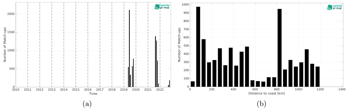
Figure 1: Number of match-ups between Saildrone and SMOS SSS L2 v700 (ESA) SSS as a function of time (a) and as function of the distance to coast (b) over the Gulf Stream Pi-MEP region and for the full satellite product period.
