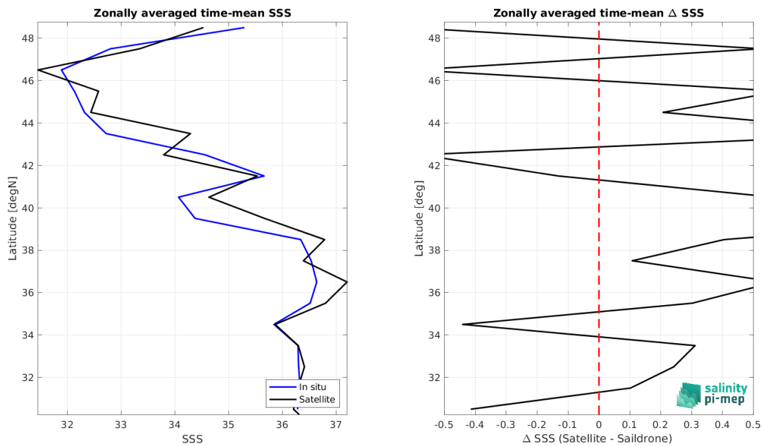
Figure 8: Left panel: Zonal mean SSS from SMOS SSS L2 v700 (ESA) satellite product (black) and from Sairdron (blue). Right panel: Zonal mean of \Delta SSS (Satellite - Sairdron) for all the collected Pi-MEP match-up pairs estimated over the full satellite product period.
