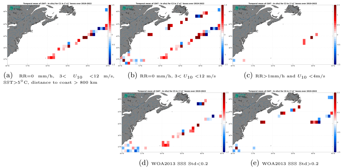
Figure 12: Temporal mean gridded over spatial boxes of size 1^\circ \times 1^\circ of \Delta SSS (SMOS SSS L2 v700 (ESA) - Sairdrone) for 5 different subdatasets corresponding to:RR=0 mm/h, 3 < U_{10} < 12 m/s, SST >5^\circ C, distance to coast > 800 km (a), RR=0 mm/h, 3 < U_{10} < 12 m/s (b), RR >1 mm/h and U_{10} < 4 m/s (c), WOA2013 SSS Std <0.2 (d), WOA2013 SSS Std >0.2 (e).
