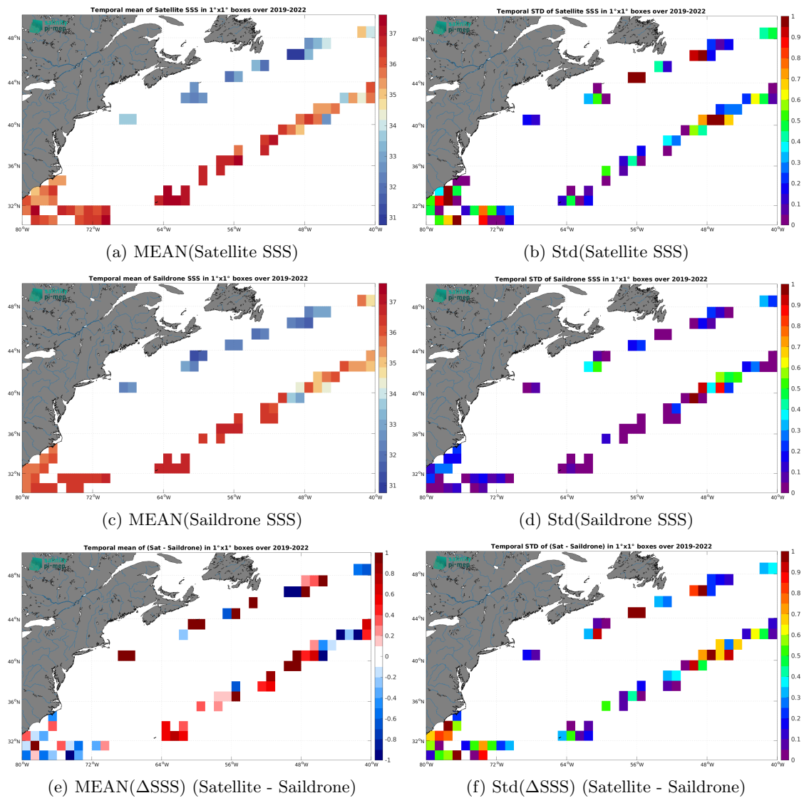
Figure 6: Temporal mean (left) and Std (right) of SSS from SMOS SSS L2 v700 (ESA) (top), Saildrone (middle), and of \Delta SSS (Satellite - Saildrone). Only match-up pairs are used to generate these maps.
