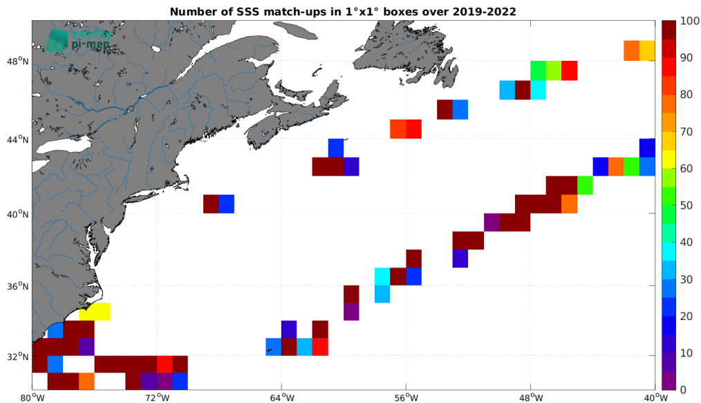
Figure 4: Number of SSS match-ups between Saildrone SSS and the SMOS SSS L2 v700 (ESA) SSS product for the Gulf Stream Pi-MEP region over 1^\circ \times 1^\circ boxes and for the full satellite product period.
