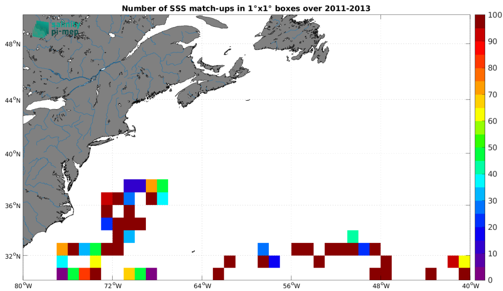
Figure 4: Number of SSS match-ups between Surface drifters SSS and the SMOS SSS L2 v700 (ESA) SSS product for the Gulf Stream Pi-MEP region over 1^\circ \times 1^\circ boxes and for the full satellite product period.
