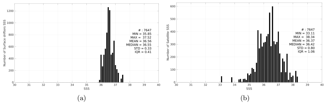
Figure 3: Histograms of SSS from Surface drifters (a) and SMOS SSS L2 v700 (ESA) (b) considering all match-up pairs per bins of 0.1 over the Gulf Stream Pi-MEP region and for the full satellite product period.
