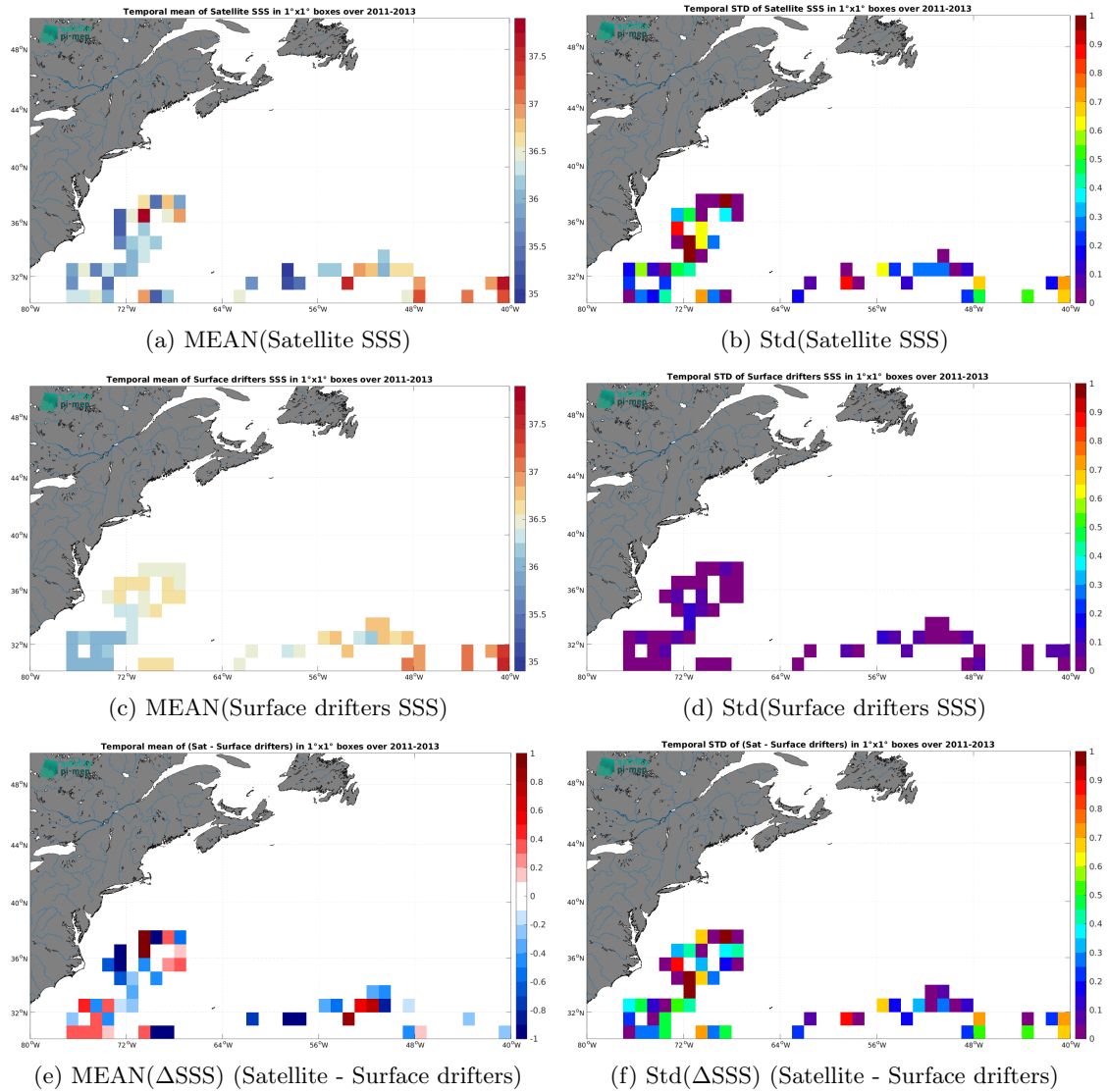
Figure 6: Temporal mean (left) and Std (right) of SSS from SMOS SSS L2 v700 (ESA) (top), Surface drifters (middle), and of \Delta SSS (Satellite - Surface drifters). Only match-up pairs are used to generate these maps.
