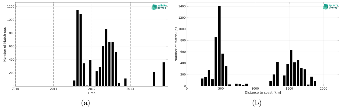
Figure 2: Number of match-ups between Surface drifters and SMOS SSS L2 v700 (ESA) SSS as a function of time (a) and as function of the distance to coast (b) over the Gulf Stream Pi-MEP region and for the full satellite product period.
