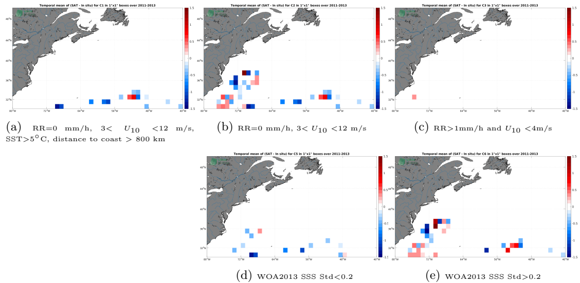
Figure 11: Temporal mean gridded over spatial boxes of size 1^{\circ}\times 1^{\circ} of \Delta\text{SSS} (SMOS SSS L2 v700 (ESA) - Surface drifters) for 5 different subdatasets corresponding to:RR=0 mm/h, 3 < U_{10} < 12 m/s, SST >5^{\circ}\text{C} , distance to coast > 800 km (a), RR=0 mm/h, 3 < U_{10} < 12 m/s (b), RR >1 mm/h and U_{10} < 4 m/s (c), WOA2013 SSS Std <0.2 (d), WOA2013 SSS Std >0.2 (e).
