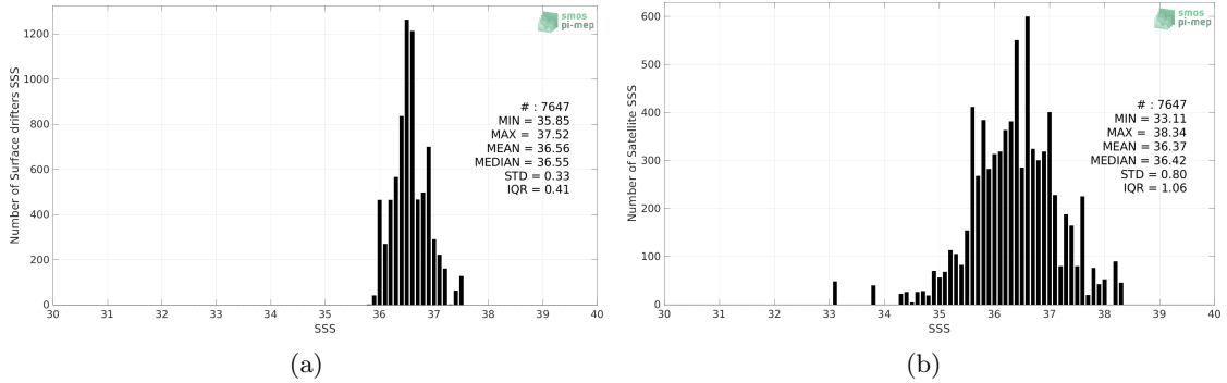
Figure 2: Histograms of SSS from Surface drifters (a) and SMOS SSS L2 v700 (ESA) (b) considering all match-up pairs per bins of 0.1 over the Gulf Stream Pi-MEP region and for the full satellite product period.
