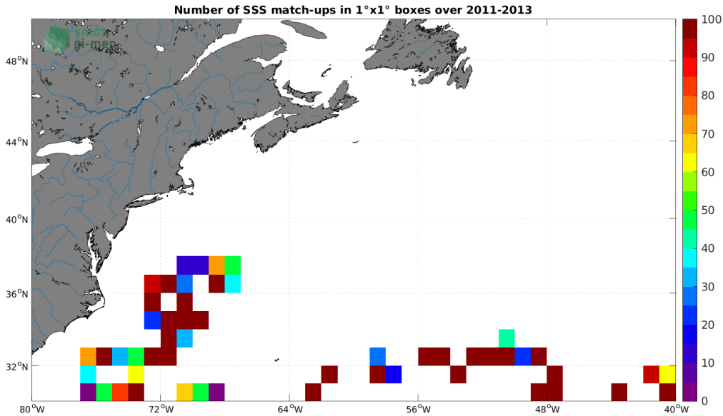
Figure 3: Number of SSS match-ups between Surface drifters SSS and the SMOS SSS L2 v700 (ESA) SSS product for the Gulf Stream Pi-MEP region over 1^\circ \times 1^\circ boxes and for the full satellite product period.
