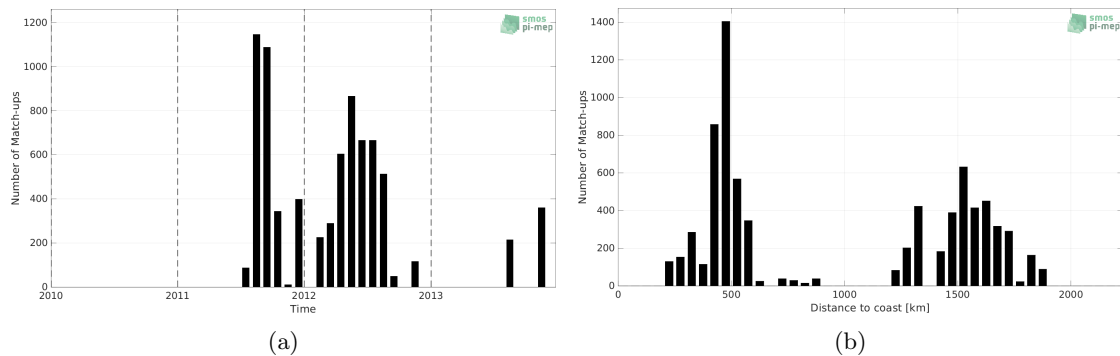
Figure 1: Number of match-ups between Surface drifters and SMOS SSS L2 v700 (ESA) SSS as a function of time (a) and as function of the distance to coast (b) over the Gulf Stream Pi-MEP region and for the full satellite product period.
