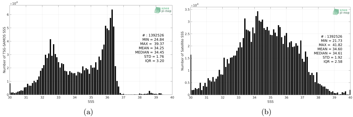
Figure 2: Histograms of SSS from TSG-SAMOS (a) and SMOS L2 v662 (ESA) (b) considering all match-up pairs per bins of 0.1 over the Gulf Stream Pi-MEP region and for the full satellite product period.
