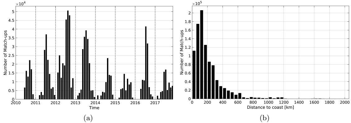
Figure 1: Number of match-ups between TSG-SAMOS and SMOS-L2-DPGS-v662 SSS as a function of time (a) and as function of the distance to coast (b) over the Gulf Stream Pi-MEP region and for the full satellite product period.
