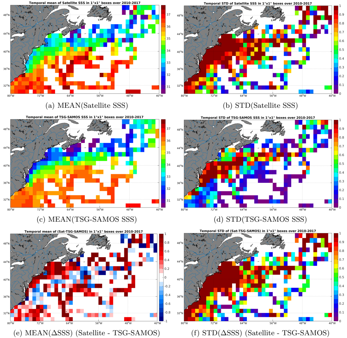
Figure 6: Temporal mean (left) and STD (right) of SSS from SMOS-L2-DPGS-v662 (top), TSG-SAMOS (middle), and of \Delta SSS (Satellite - TSG-SAMOS). Only match-up pairs are used to generate these maps.
