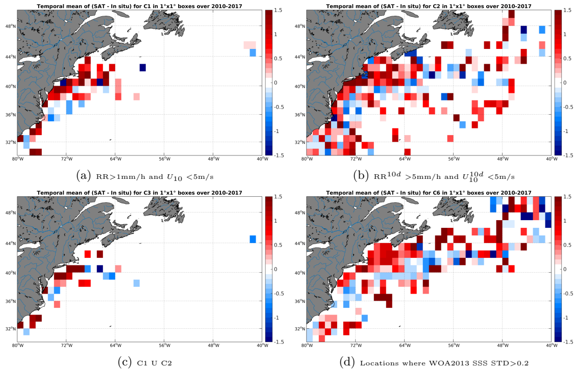
Figure 12: Temporal mean gridded over spatial boxes of size 1^\circ \times 1^\circ of \Delta SSS (SMOS-L2-DPGS-v662 - TSG-SAMOS) for 4 different subdatasets corresponding to: RR > 1\text{mm/h} and U_{10} < 5\text{m/s} (a), RR^{10d} > 5\text{mm/h} and U_{10}^{10d} < 5\text{m/s} (b), C1 U C2 (c), Locations where WOA2013 SSS STD > 0.2 (d).
