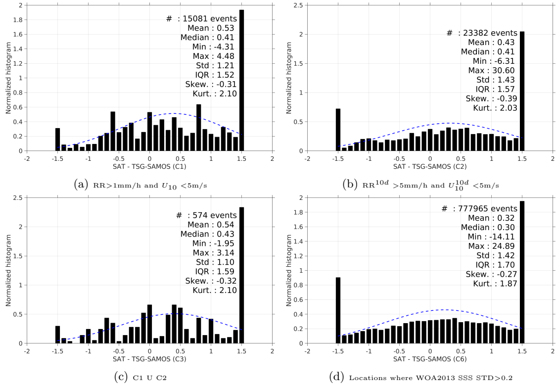
Figure 13: Normalized histogram of \Delta SSS (SMOS-L2-DPGS-v662 - TSG-SAMOS) for 6 different subdatasets corresponding to: RR > 1\text{mm/h} and U_{10} < 5\text{m/s} (a), RR^{10d} > 5\text{mm/h} and U_{10}^{10d} < 5\text{m/s} (b), C1 \cup C2 (c), Locations where WOA2013 SSS STD > 0.2 (d).
