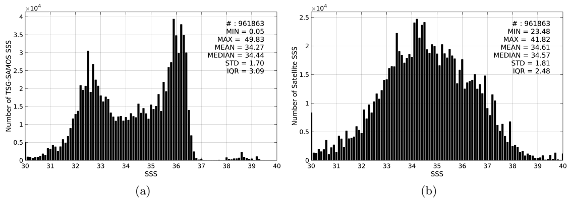
Figure 2: Histograms of SSS from TSG-SAMOS (a) and SMOS-L2-DPGS-v662 (b) considering all match-up pairs per bins of 0.1 over the Gulf Stream Pi-MEP region and for the full satellite product period.
