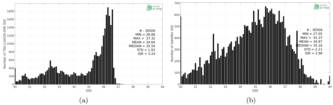
Figure 2: Histograms of SSS from TSG (LEGOS-DM) (a) and SMOS SSS L2 v662 (ESA) (b) considering all match-up pairs per bins of 0.1 over the Gulf Stream Pi-MEP region and for the full satellite product period.
