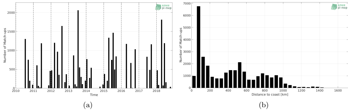
Figure 1: Number of match-ups between TSG (LEGOS-DM) and SMOS SSS L2 v662 (ESA) SSS as a function of time (a) and as function of the distance to coast (b) over the Gulf Stream Pi-MEP region and for the full satellite product period.
