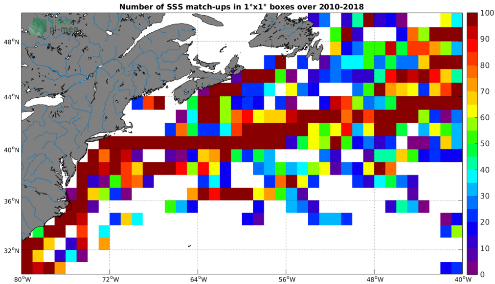
Figure 4: Number of SSS match-ups between TSG (LEGOS-DM) SSS and the SMOS SSS L2 v662 (ESA) SSS product for the Gulf Stream Pi-MEP region over 1^\circ \times 1^\circ boxes and for the full satellite product period.
