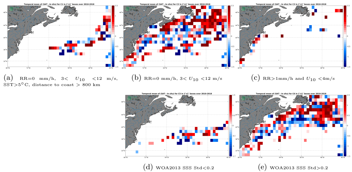
Figure 12: Temporal mean gridded over spatial boxes of size 1^\circ \times 1^\circ of \Delta SSS (SMOS SSS L2 v662 (ESA) - TSG (LEGOS-DM)) for 5 different subdatasets corresponding to:RR=0 mm/h, 3 < U_{10} < 12 m/s, SST >5^\circ\text{C} , distance to coast > 800 km (a), RR=0 mm/h, 3 < U_{10} < 12 m/s (b), RR >1 mm/h and U_{10} < 4 m/s (c), WOA2013 SSS Std <0.2 (d), WOA2013 SSS Std >0.2 (e).
