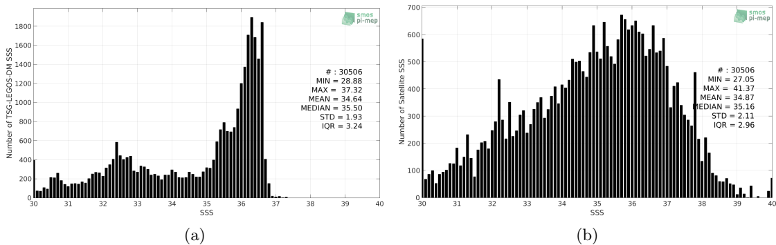
Figure 2: Histograms of SSS from TSG-LEGOS-DM (a) and SMOS L2 v662 (ESA) (b) considering all match-up pairs per bins of 0.1 over the Gulf Stream Pi-MEP region and for the full satellite product period.
