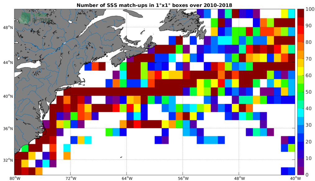
Figure 4: Number of SSS match-ups between TSG-LEGOS-DM SSS and the SMOS L2 v662 (ESA) SSS product for the Gulf Stream Pi-MEP region over 1^\circ \times 1^\circ boxes and for the full satellite product period.
