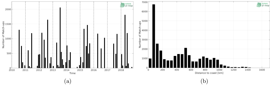
Figure 1: Number of match-ups between TSG-LEGOS-DM and SMOS L2 v662 (ESA) SSS as a function of time (a) and as function of the distance to coast (b) over the Gulf Stream Pi-MEP region and for the full satellite product period.
