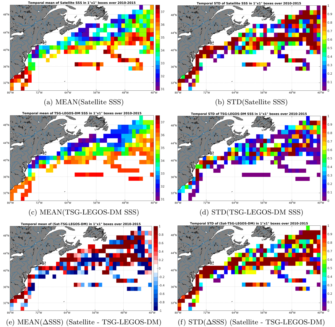
Figure 6: Temporal mean (left) and STD (right) of SSS from SMOS-L2-DPGS-v662 (top), TSG-LEGOS-DM (middle), and of \Delta SSS (Satellite - TSG-LEGOS-DM). Only match-up pairs are used to generate these maps.
