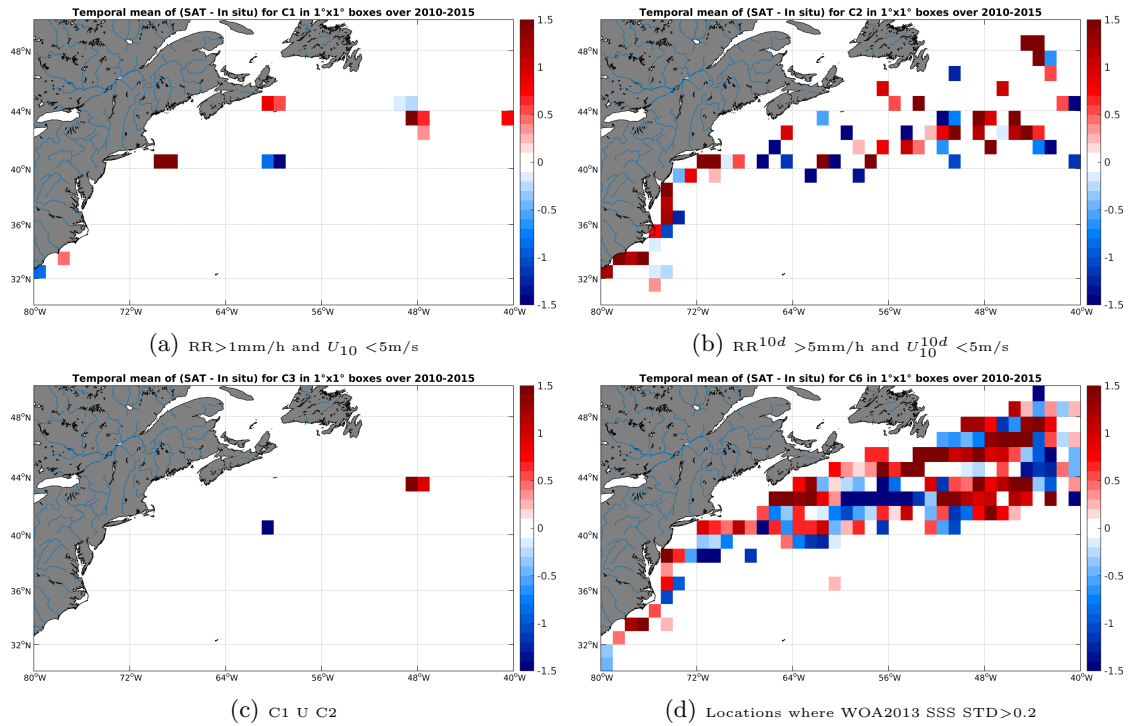
Figure 12: Temporal mean gridded over spatial boxes of size 1°x1° of \Delta SSS (SMOS-L2-DPGS-v662 - TSG-LEGOS-DM) for 4 different subdatasets corresponding to:RR>1mm/h and U_{10} < 5 m/s (a), RR^{10d} > 5 mm/h and U_{10}^{10d} < 5 m/s (b), C1 U C2 (c),Locations where WOA2013 SSS STD>0.2 (d).
