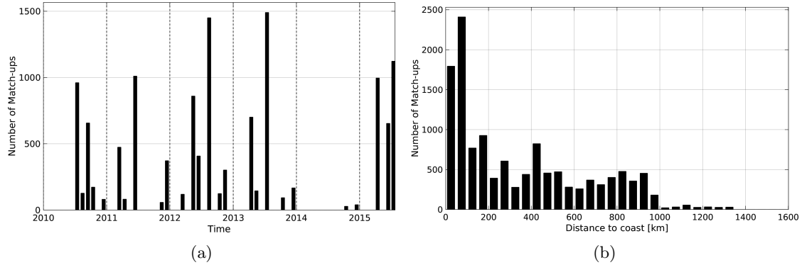
Figure 1: Number of match-ups between TSG-LEGOS-DM and SMOS-L2-DPGS-v662 SSS as a function of time (a) and as function of the distance to coast (b) over the Gulf Stream Pi-MEP region and for the full satellite product period.
