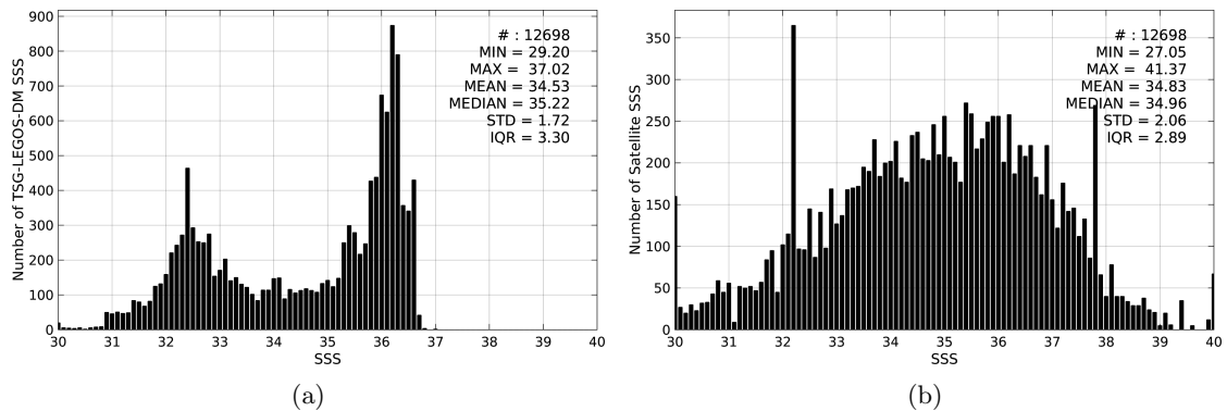
Figure 2: Histograms of SSS from TSG-LEGOS-DM (a) and SMOS-L2-DPGS-v662 (b) considering all match-up pairs per bins of 0.1 over the Gulf Stream Pi-MEP region and for the full satellite product period.
