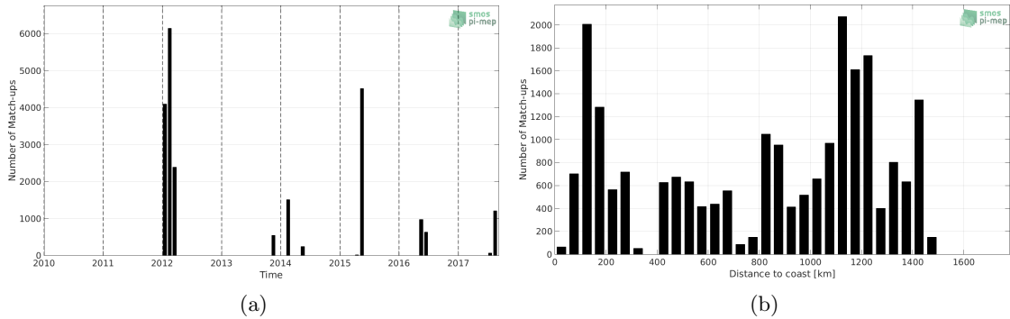
Figure 1: Number of match-ups between TSG (GOSUD-Sailing-ship) and SMOS SSS L2 v662 (ESA) SSS as a function of time (a) and as function of the distance to coast (b) over the Gulf Stream Pi-MEP region and for the full satellite product period.
