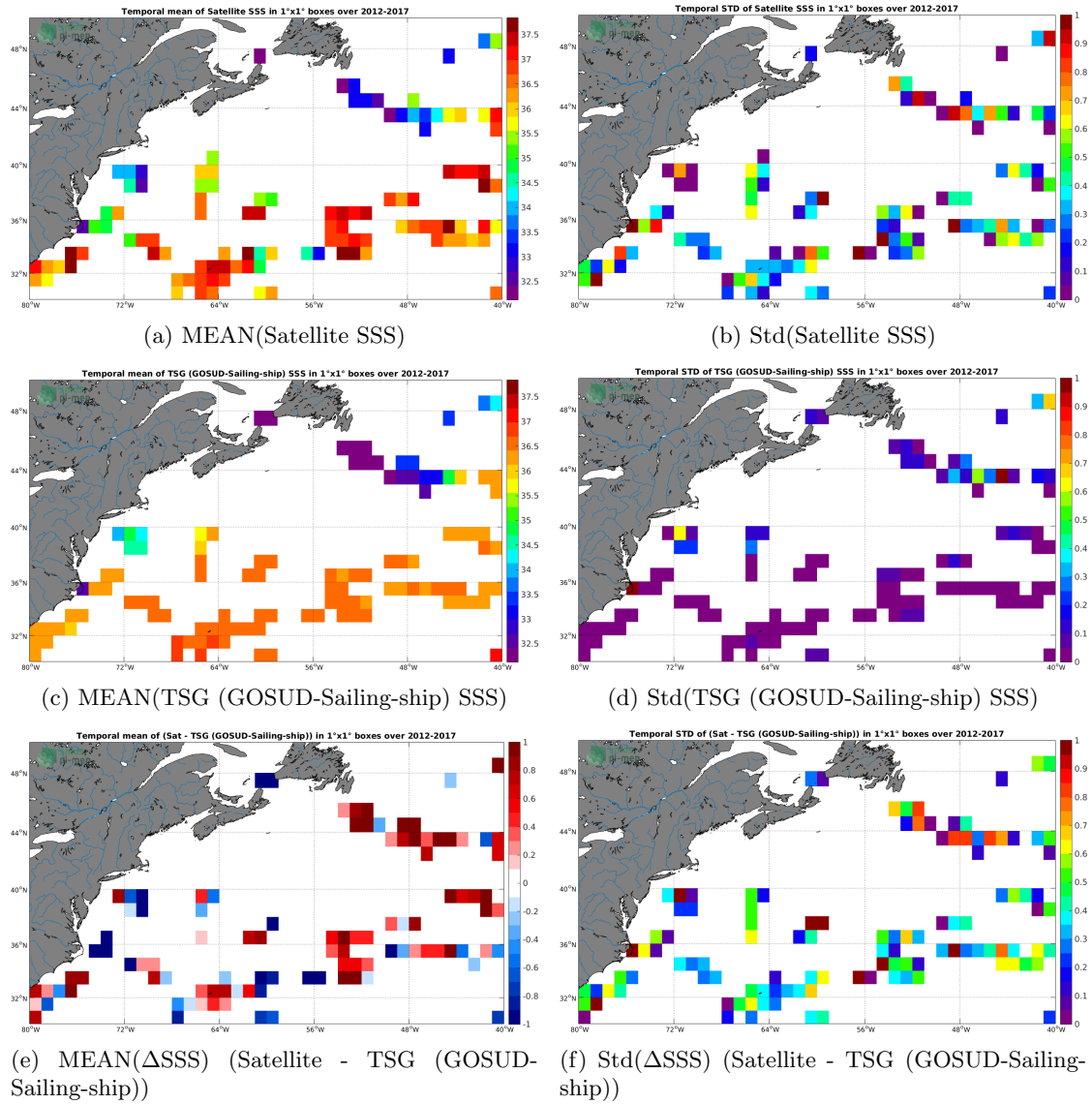
Figure 6: Temporal mean (left) and Std (right) of SSS from SMOS SSS L2 v662 (ESA) (top), TSG (GOSUD-Sailing-ship) (middle), and of \Delta SSS (Satellite - TSG (GOSUD-Sailing-ship)). Only match-up pairs are used to generate these maps.
