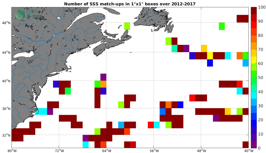
Figure 4: Number of SSS match-ups between TSG (GOSUD-Sailing-ship) SSS and the SMOS SSS L2 v662 (ESA) SSS product for the Gulf Stream Pi-MEP region over 1°x1° boxes and for the full satellite product period.
