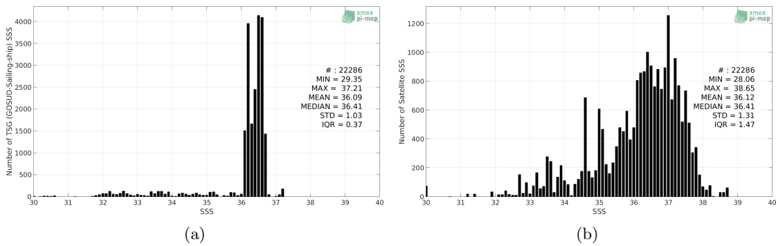
Figure 2: Histograms of SSS from TSG (GOSUD-Sailing-ship) (a) and SMOS SSS L2 v662 (ESA) (b) considering all match-up pairs per bins of 0.1 over the Gulf Stream Pi-MEP region and for the full satellite product period.
