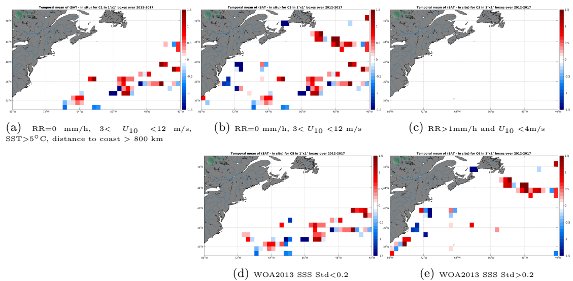
Figure 12: Temporal mean gridded over spatial boxes of size 1°x1° of \Delta SSS (SMOS SSS L2 v662 (ESA) - TSG (GOSUD-Sailing-ship)) for 5 different subdatasets corresponding to: RR=0 mm/h, 3 < U_{10} < 12 m/s, SST > 5°C, distance to coast > 800 km (a), RR=0 mm/h, 3 < U_{10} < 12 m/s (b), RR > 1 mm/h and U_{10} < 4 m/s (c), WOA2013 SSS Std < 0.2 (d), WOA2013 SSS Std > 0.2 (e).
