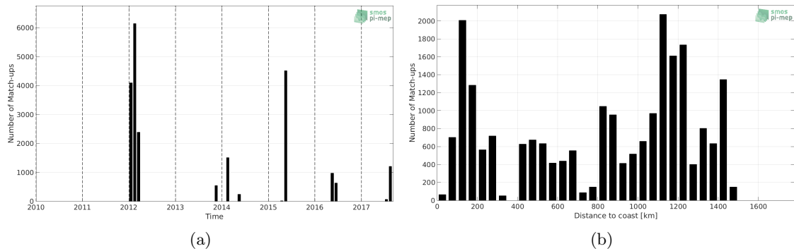
Figure 1: Number of match-ups between TSG-GOSUD-Sailing-ship and SMOS L2 v662 (ESA) SSS as a function of time (a) and as function of the distance to coast (b) over the Gulf Stream Pi-MEP region and for the full satellite product period.
