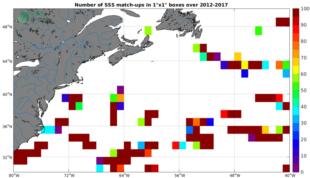
Figure 4: Number of SSS match-ups between TSG-GOSUD-Sailing-ship SSS and the SMOS L2 v662 (ESA) SSS product for the Gulf Stream Pi-MEP region over 1^\circ \times 1^\circ boxes and for the full satellite product period.
