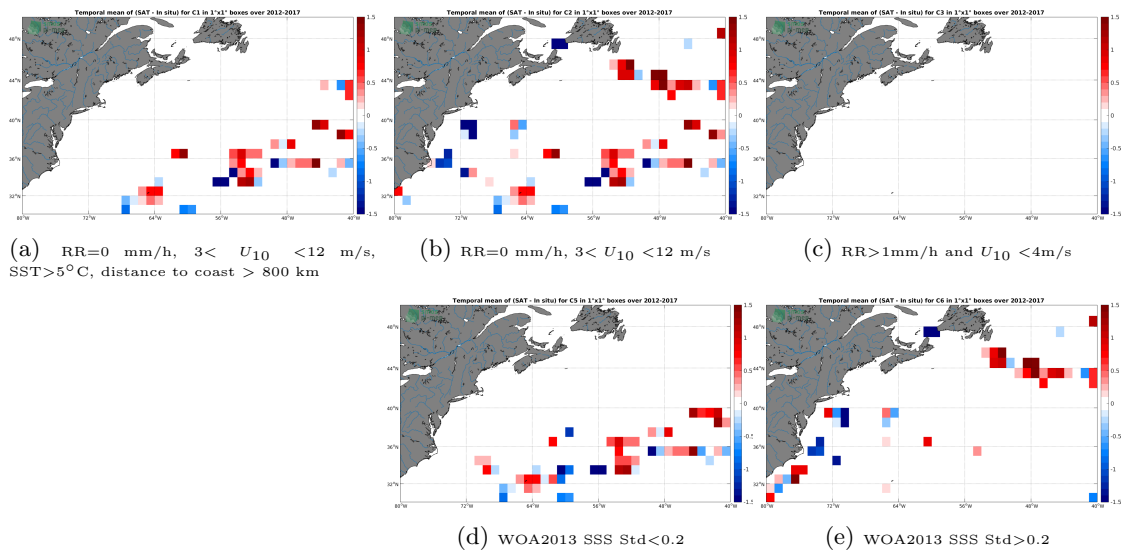
Figure 12: Temporal mean gridded over spatial boxes of size 1°x1° of \Delta SSS (SMOS L2 v662 (ESA) - TSG-GOSUD-Sailing-ship) for 5 different subdatasets corresponding to:RR=0 mm/h, 3 < U_{10} < 12 m/s, SST > 5°C, distance to coast > 800 km (a), RR=0 mm/h, 3 < U_{10} < 12 m/s (b), RR > 1mm/h and U_{10} < 4m/s (c), WOA2013 SSS Std < 0.2 (d), WOA2013 SSS Std > 0.2 (e).
