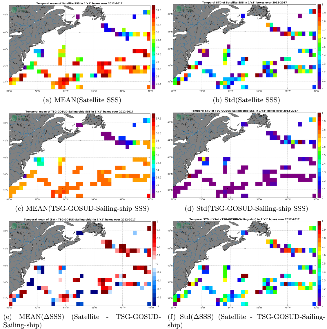
Figure 6: Temporal mean (left) and Std (right) of SSS from SMOS L2 v662 (ESA) (top), TSG-GOSUD-Sailing-ship (middle), and of \Delta SSS (Satellite - TSG-GOSUD-Sailing-ship). Only match-up pairs are used to generate these maps.
