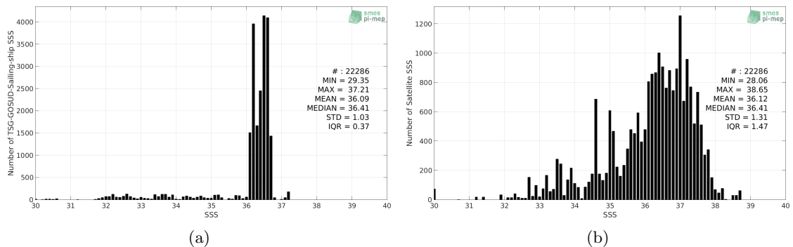
Figure 2: Histograms of SSS from TSG-GOSUD-Sailing-ship (a) and SMOS L2 v662 (ESA) (b) considering all match-up pairs per bins of 0.1 over the Gulf Stream Pi-MEP region and for the full satellite product period.
