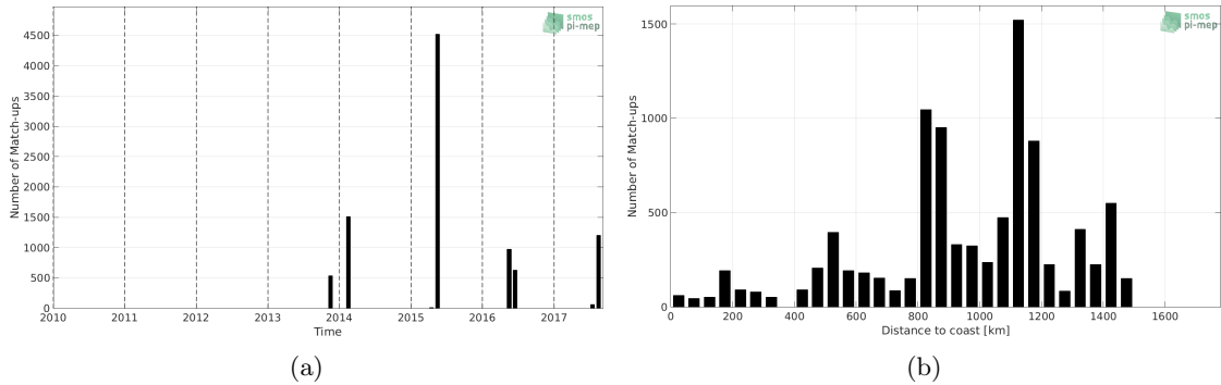
Figure 1: Number of match-ups between TSG-GOSUD-Sailing-ship and SMOS-L2-DPGS-v662 SSS as a function of time (a) and as function of the distance to coast (b) over the Gulf Stream Pi-MEP region and for the full satellite product period.
