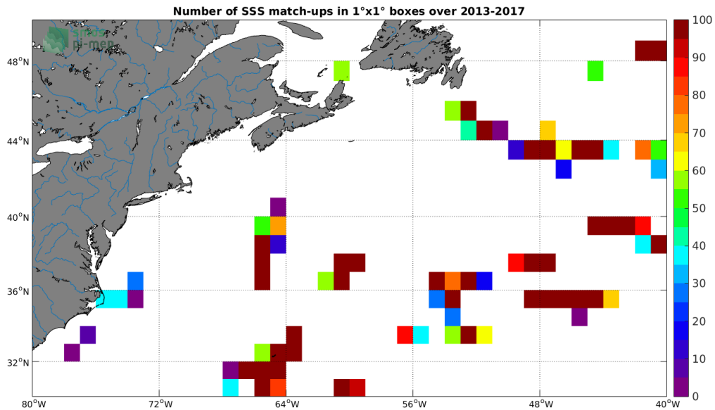
Figure 4: Number of SSS match-ups between TSG-GOSUD-Sailing-ship SSS and the SMOS-L2-DPGS-v662 SSS product for the Gulf Stream Pi-MEP region over 1^\circ \times 1^\circ boxes and for the full satellite product period.
