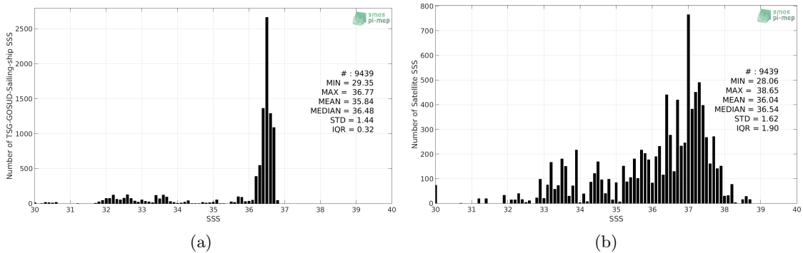
Figure 2: Histograms of SSS from TSG-GOSUD-Sailing-ship (a) and SMOS-L2-DPGS-v662 (b) considering all match-up pairs per bins of 0.1 over the Gulf Stream Pi-MEP region and for the full satellite product period.
