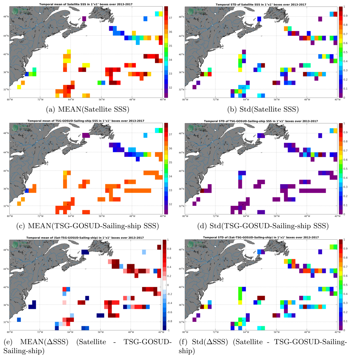
Figure 6: Temporal mean (left) and Std (right) of SSS from SMOS-L2-DPGS-v662 (top), TSG-GOSUD-Sailing-ship (middle), and of \Delta SSS (Satellite - TSG-GOSUD-Sailing-ship). Only match-up pairs are used to generate these maps.
