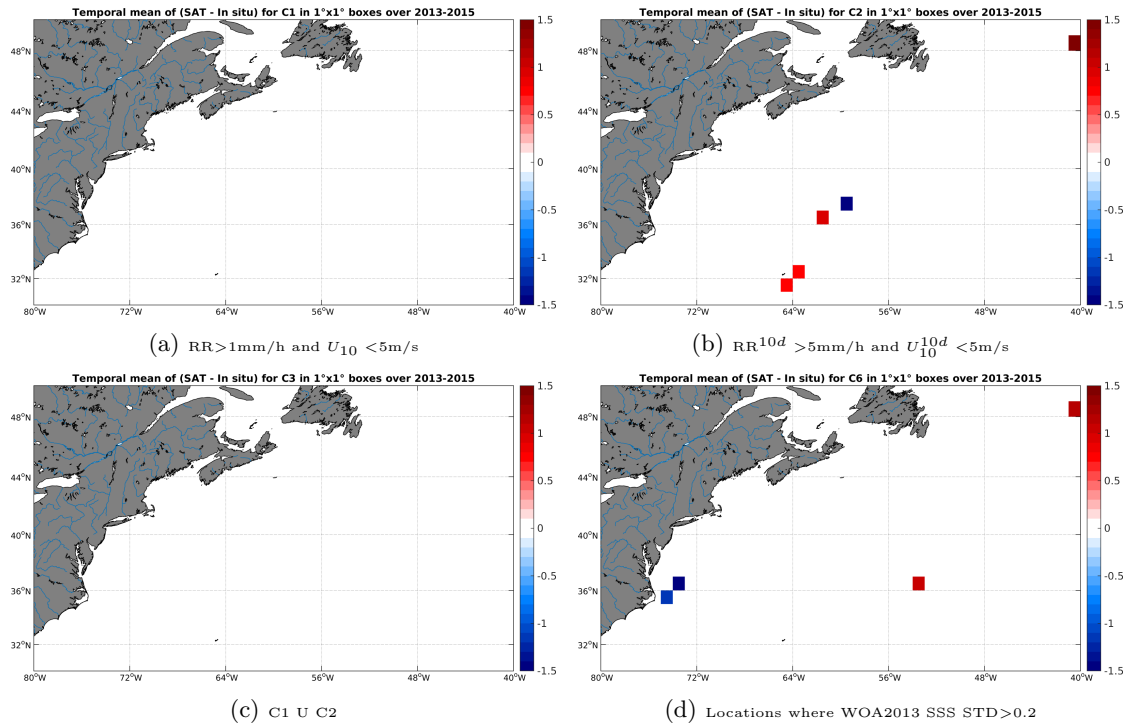
Figure 12: Temporal mean gridded over spatial boxes of size 1^\circ \times 1^\circ of \Delta SSS (SMOS-L2-DPGS-v662 - TSG-GOSUD-Sailing-ship) for 4 different subdatasets corresponding to:RR >1 mm/h and U_{10} < 5 m/s (a), RR^{10d} > 5 mm/h and U_{10}^{10d} < 5 m/s (b), C1 U C2 (c),Locations where WOA2013 SSS STD >0.2 (d).
