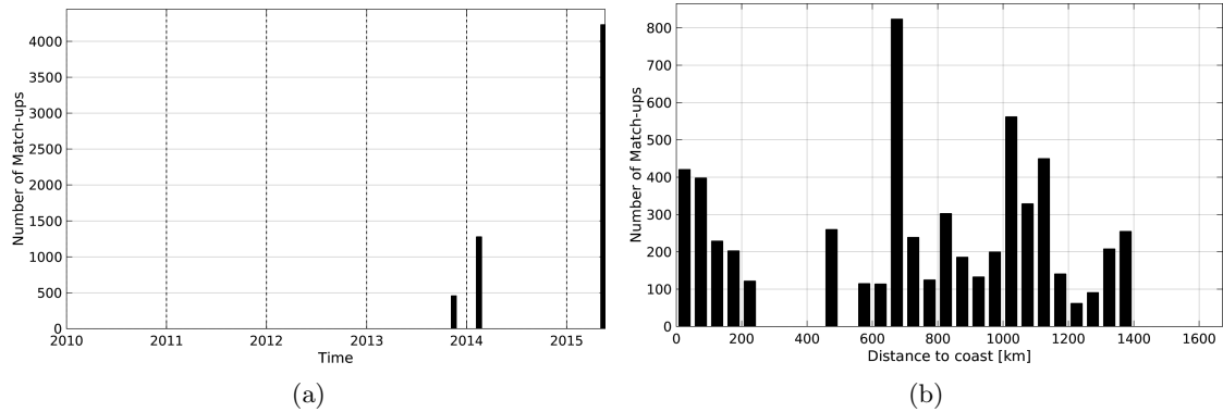
Figure 1: Number of match-ups between TSG-GOSUD-Sailing-ship and SMOS-L2-DPGS-v662 SSS as a function of time (a) and as function of the distance to coast (b) over the Gulf Stream Pi-MEP region and for the full satellite product period.
