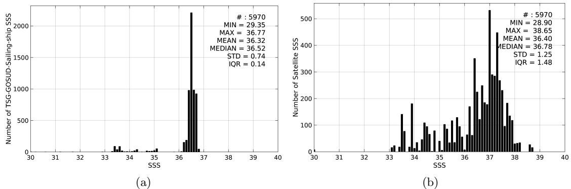
Figure 2: Histograms of SSS from TSG-GOSUD-Sailing-ship (a) and SMOS-L2-DPGS-v662 (b) considering all match-up pairs per bins of 0.1 over the Gulf Stream Pi-MEP region and for the full satellite product period.
