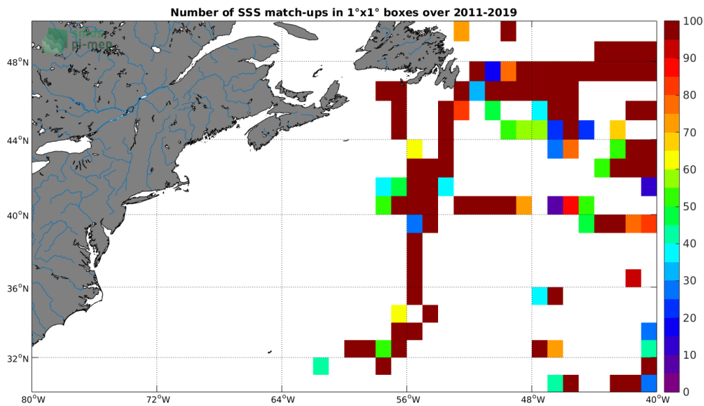
Figure 4: Number of SSS match-ups between TSG (GOSUD-Research-vessel) SSS and the SMOS SSS L2 v662 (ESA) SSS product for the Gulf Stream Pi-MEP region over 1^\circ \times 1^\circ boxes and for the full satellite product period.
