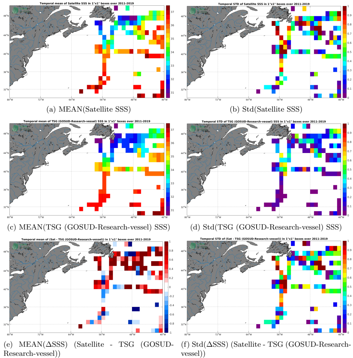
Figure 6: Temporal mean (left) and Std (right) of SSS from SMOS SSS L2 v662 (ESA) (top), TSG (GOSUD-Research-vessel) (middle), and of \Delta SSS (Satellite - TSG (GOSUD-Research-vessel)). Only match-up pairs are used to generate these maps.
