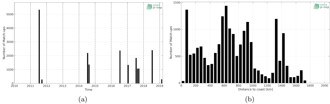
Figure 1: Number of match-ups between TSG (GOSUD-Research-vessel) and SMOS SSS L2 v662 (ESA) SSS as a function of time (a) and as function of the distance to coast (b) over the Gulf Stream Pi-MEP region and for the full satellite product period.
