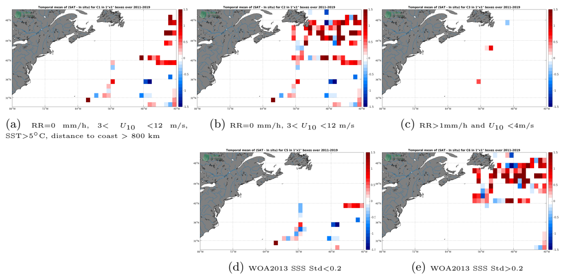
Figure 12: Temporal mean gridded over spatial boxes of size 1°x1° of \Delta SSS (SMOS SSS L2 v662 (ESA) - TSG (GOSUD-Research-vessel)) for 5 different subdatasets corresponding to:RR=0 mm/h, 3 < U_{10} < 12 m/s, SST > 5°C, distance to coast > 800 km (a), RR=0 mm/h, 3 < U_{10} < 12 m/s (b), RR > 1mm/h and U_{10} < 4 m/s (c), WOA2013 SSS Std < 0.2 (d), WOA2013 SSS Std > 0.2 (e).
