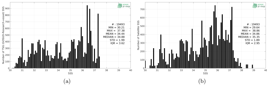
Figure 2: Histograms of SSS from TSG (GOSUD-Research-vessel) (a) and SMOS SSS L2 v662 (ESA) (b) considering all match-up pairs per bins of 0.1 over the Gulf Stream Pi-MEP region and for the full satellite product period.
